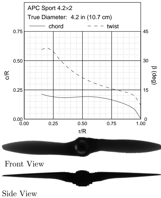
Figure 6: APC Sport 4.2x2 geometric characteristics.
