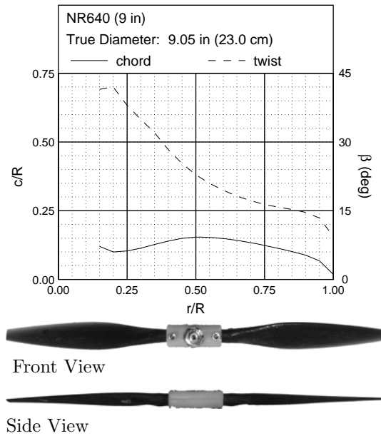
Figure 10: 9 in NR640 geometric characteristics.
