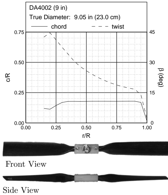
Figure 8: 9 in DA4002 geometric characteristics.
