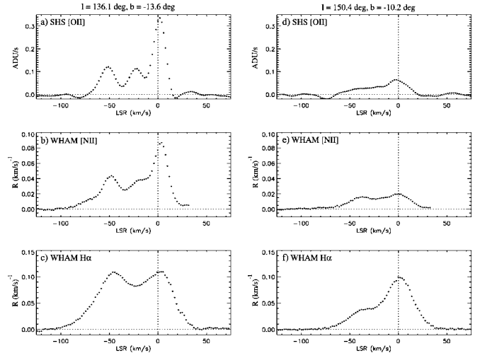
FIG. 2.—SHS [O II] spectra and WHAM [N II] and H\alpha spectra toward two directions that sample warm ionized gas in both the local and Perseus spiral arms. Toward l = 136.1^\circ , b = -13.6^\circ (left) the spectra clearly show that the local gas (component near 0 \text{ km s}^{-1} ) has elevated [O II]/ H\alpha and [N II]/ H\alpha , implying a higher temperature, compared to the local component toward l = 150.4^\circ , b = -10.2^\circ (right). Intensity scales for the WHAM H\alpha and [N II] observations are in R \text{ (km s}^{-1}\text{)}^{-1} ; the SHS [O II] intensity is in arbitrary units (but consistent between [O II] spectra).
