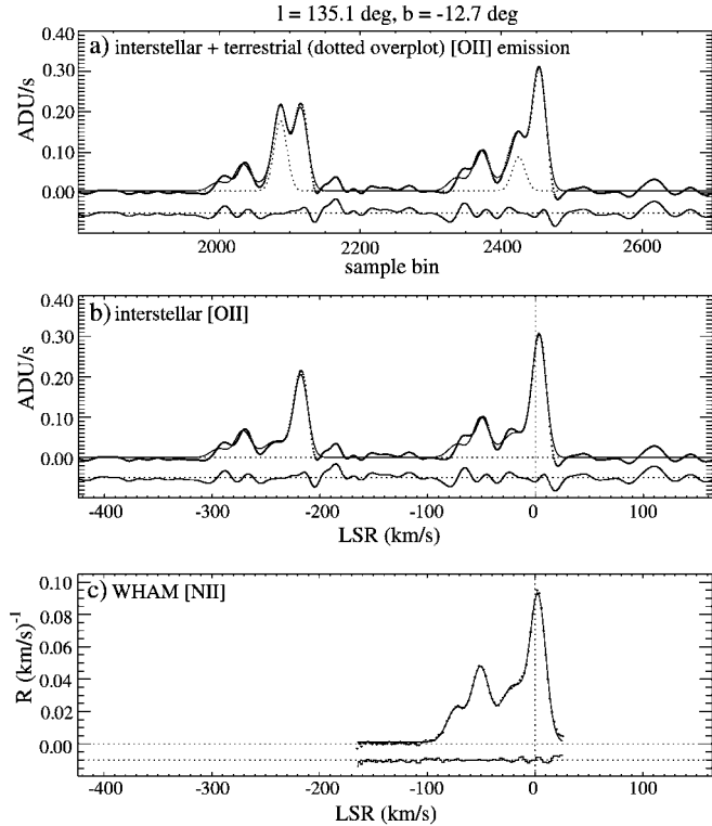
FIG. 1.—Example fit to an [O II] SHS spectrum. (a) Fitted [O II] emission (solid line). (b) Diffuse Galactic [O II] emission free of terrestrial [O II] contributions; emission along the lines of sight from both the local and more distant gas in the Perseus spiral arm (Doppler shifted \sim 40 \text{ km s}^{-1} to the blue), is apparent. Note the velocity scale for [O II] is referenced to the 3729 \text{ \AA} line of the doublet. (c) WHAM [N II] spectrum. The intensity scale for the WHAM [N II] observation (c) is in R \text{ (km s}^{-1}\text{)}^{-1} ; the SHS [O II] intensity (panels a and b) is in arbitrary units (but consistent between [O II] spectra).
