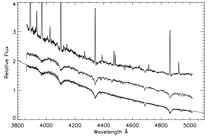
FIG. 9.—Bok 2.4 m emission-line spectra at the superior conjunction ( top ) compared with the spectrum at the inferior conjunction ( middle ) and the extracted white dwarf spectrum ( bottom ). The best-fitting model white dwarf spectrum of T_{\text{eff}} = 70,000 K and \log g = 7.75 is overplotted on top of the extracted white dwarf spectrum.
