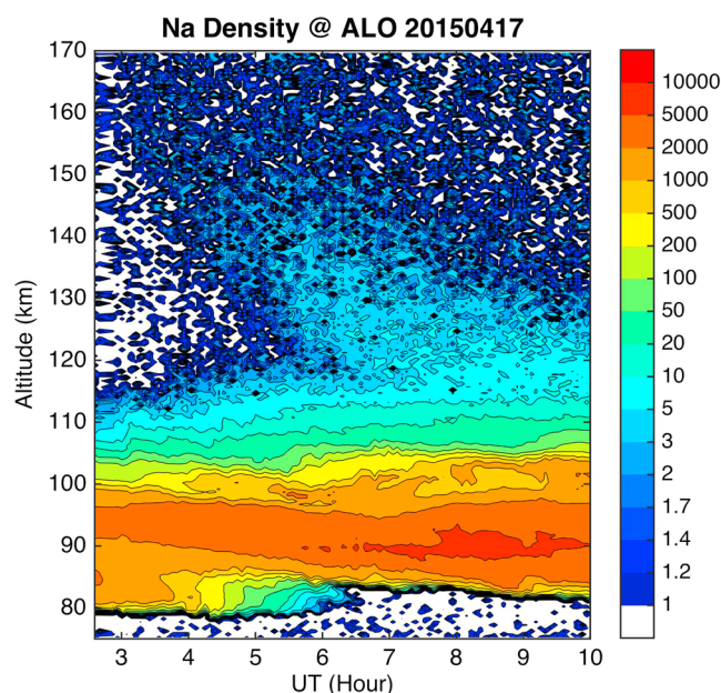
Figure 1. Na density (atoms per cm 3 ) on the night of 17 April 2015 measured by the Na lidar at Andes Lidar Observatory in Cerro Pachón, Chile. Nonlinear color scale is used to highlight the low density in the thermosphere.
