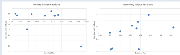
Figure 4. The residuals for the expected minima of each eclipse of EPIC 21139989 suggest that the second order polynomial used to determine the period timing was fairly accurate, with a standard deviation for the primary eclipse residuals of 0.01011 and a standard deviation for the secondary eclipse residuals of 0.00983.
