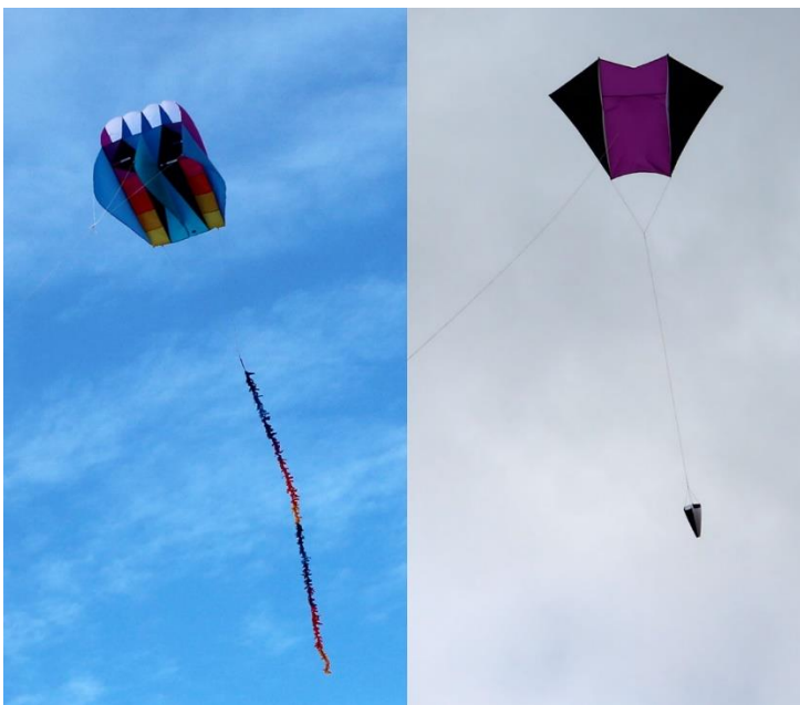
Figure 3. Two examples of tethered kites. The kite on the left is a soft kite that can fly in winds between 5 and 30 mph, although higher speeds of 15mph or more are necessary to lift a camera rig. The kite on the right is a rigid kite that has carbon fiber spars to add support. This allows the kite to fly and lift a camera rig in lower windspeeds of around 10 miles per hour or more. Higher windspeeds of 20mph or more can damage the carbon fiber spars.
