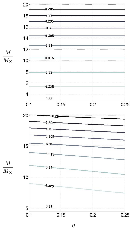
Figure 2. The ratio C_2(\eta)/i^{\eta\eta} (top) and C_2(M)/i^{M M} (bottom)
