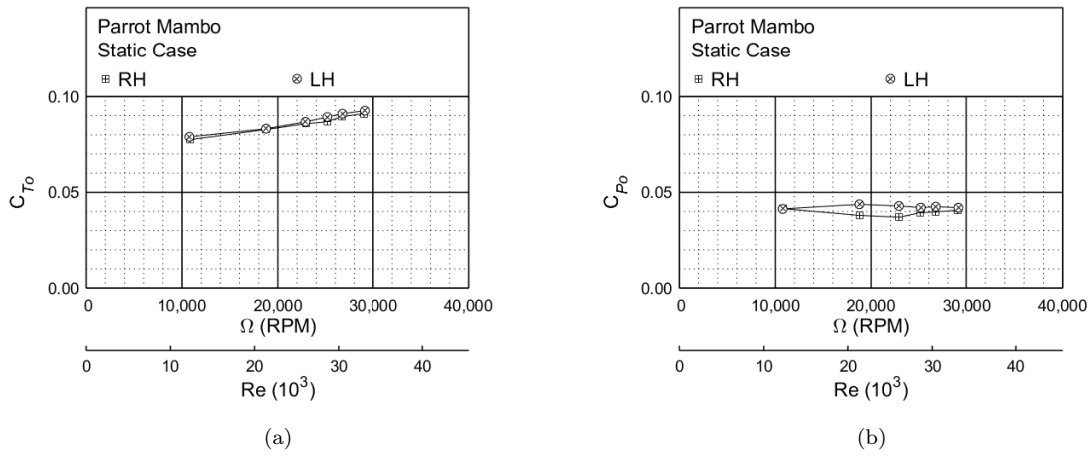
Figure 26: Static performance of the right-handed and left-handed propellers of the Parrot Mambo: (a) thrust coefficient and (b) power coefficient.
