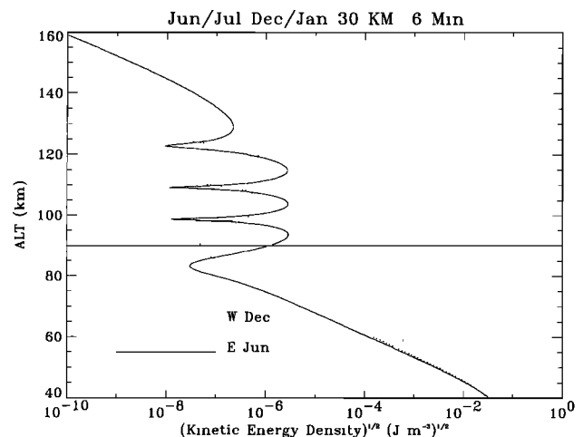
Figure 14. Plots of the kinetic energy density for two cases. An eastward wave in June/July and a westward wave in December/January.
