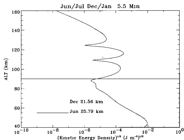
Figure 8. A plot of the kinetic energy density of the wave as a function of altitude for the waves considered in Figure 7.
