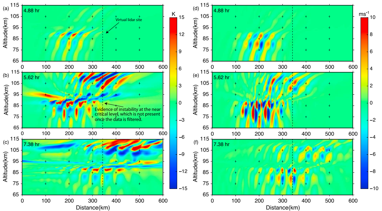
Figure 8. The original simulated (a–c) temperature and (d–f) vertical wind perturbations at t = 4.88, 5.62, and 7.38 h. Please note that the virtual lidar site is at x = 340 km and denoted by the vertical dashed line.
