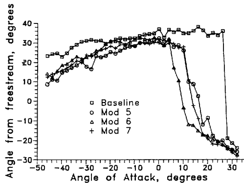
b) Resultant force direction
