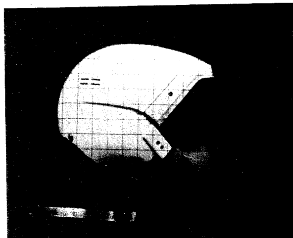
Fig. 4 Prototype helmet installed on cradle/headform assembly.
