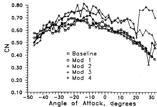
b) Normal force coefficient
