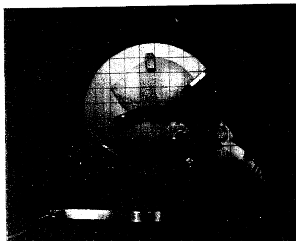
Fig. 3 Air Force helmet installed on cradle/headform assembly.
