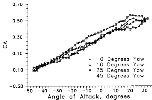
Fig. 9 Navy baseline helmet axial force change with yaw.
