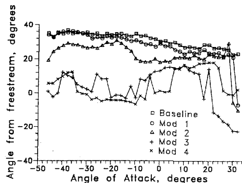
c) Resultant force angle
