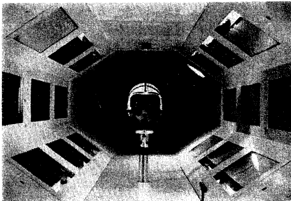
Fig. 1 Navy helmet mounted in wind tunnel.
