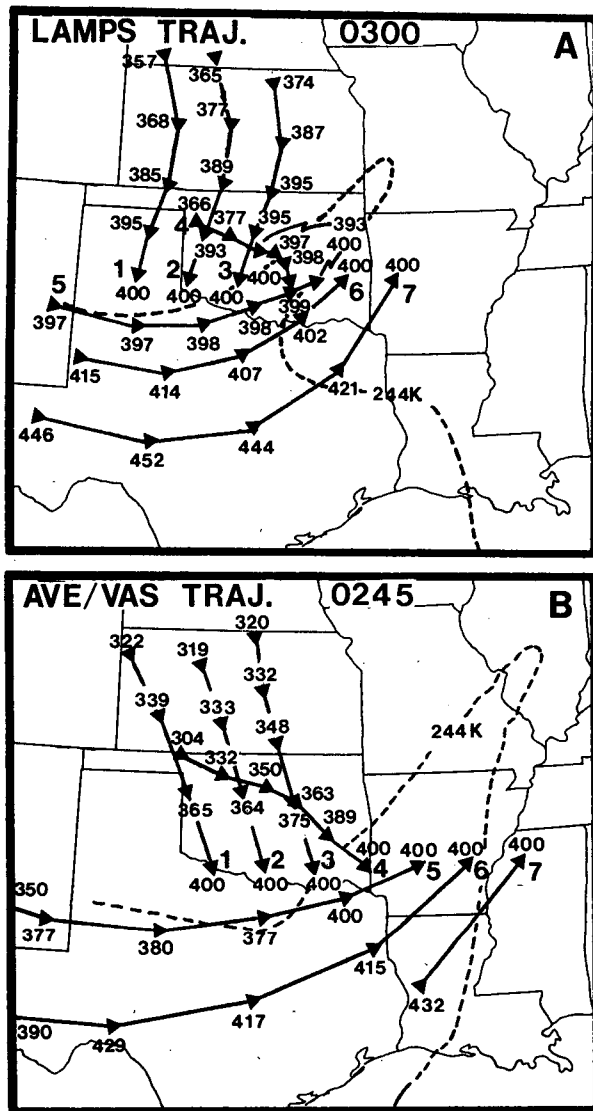
FIG. 11. (a) LAMPS trajectories ending at 400 mb on 0300 UTC 7 March computed over 3 hour increments. In both A and B, vertical positions of parcels are given in mb while dashed lines indicate the 244 K T_p contour. (b) AVE/VAS trajectories ending at 400 mb on 0245 UTC 7 March computed for time increments corresponding to the RAOB times.
