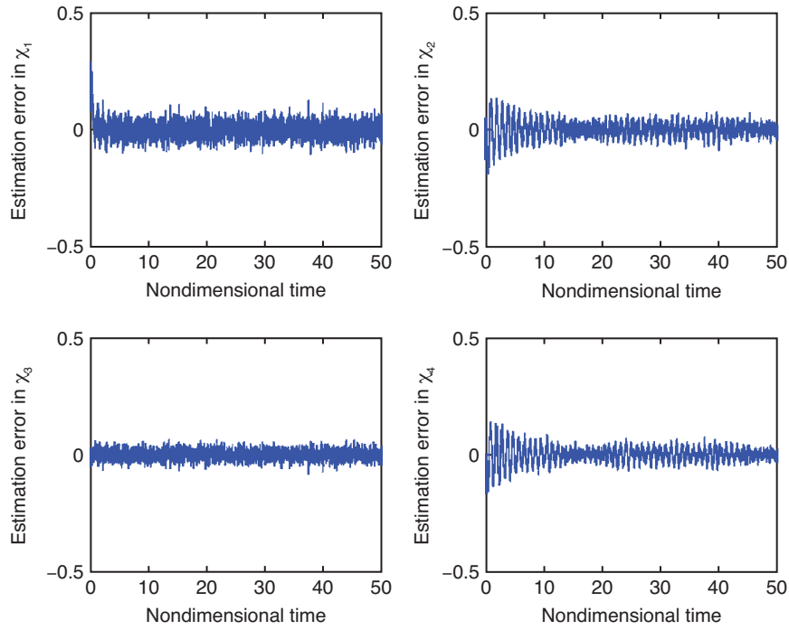
Figure 12: Time response of estimation errors \tilde{\chi} (pressure sensor).
