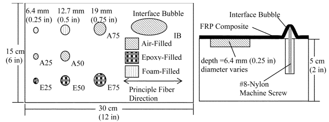
Fig. 1—Defect configuration for Series A specimens.
