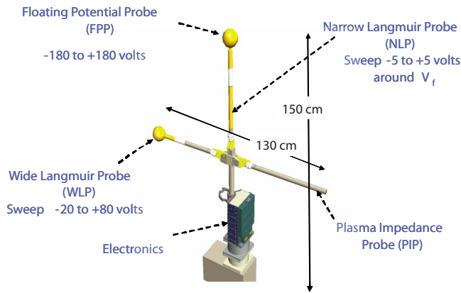
FIG. 1. (Color online) FPMU conceptual instrument layout.
