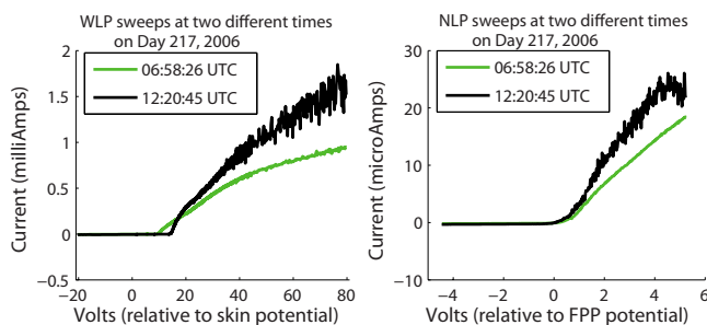
FIG. 4. (Color online) Noise in the WLP and the NLP I - V curves possibly due to interference from some other apparatus or activity onboard the ISS. Both curves are from when ISS was in eclipse conditions. The difference in floating potential observed in WLP curves is because of ISS charging due to V \times B effect.
