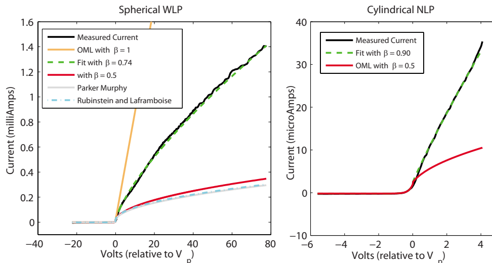
FIG. 7. (Color online) Comparison of measured I - V curves with the I - V curves generated by analytical theory. The best match is acquired with a least-squares fit of Eq. (3) to n_e and \beta . It is important to note that the fit value of \beta is different from that proposed by OML theory.
