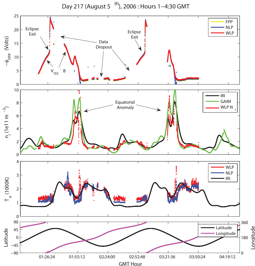
FIG. 11. (Color) The first row shows FPMU floating potential as measured by the FPP, the WLP, and the NLP. The second row compares the ion density ( n_i ) derived from the WLP with density from USU-GAIM and IRI model runs. The third row compares the WLP and the NLP derived temperatures with IRI model results. The fourth row shows the ISS latitude and longitude.
