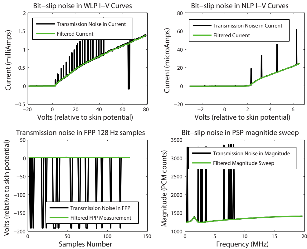
FIG. 3. (Color online) Noise in the data set of all four FPMU instruments due to telemetry errors. Median filtering mitigates most of the “spikes.”
