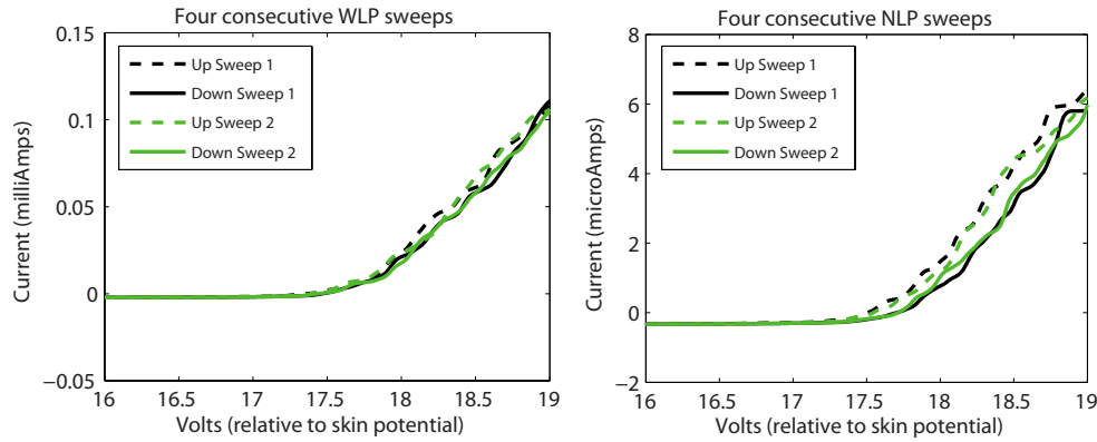
FIG. 5. (Color online) Four consecutive I - V curves from the WLP and the NLP. There is no hysteresis in the internally heated WLP, while minimal hysteresis exists in the NLP indicating presence of some contamination.
