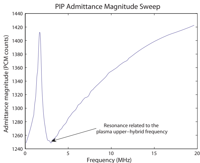
FIG. 8. (Color online) A single admittance vs frequency profile from the PIP data set.
