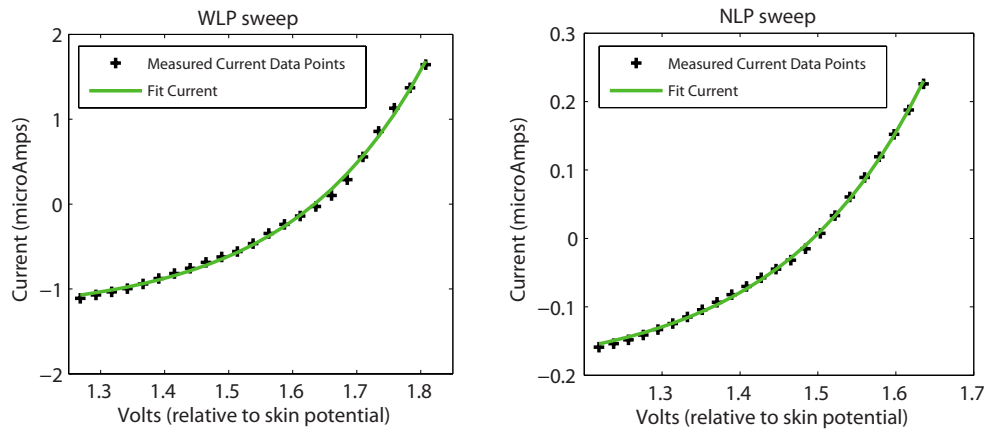
FIG. 6. (Color online) Fits for T_e and \phi_p to the electron retardation region using Eq. (7). Both the WLP and the NLP I - V curves are for the same second of data. The T_e and \phi_p fits for the WLP I - V curve were 2420 °K and 2.12 V, while for the NLP I - V curve were 2670 °K and 2.01 V, respectively.
