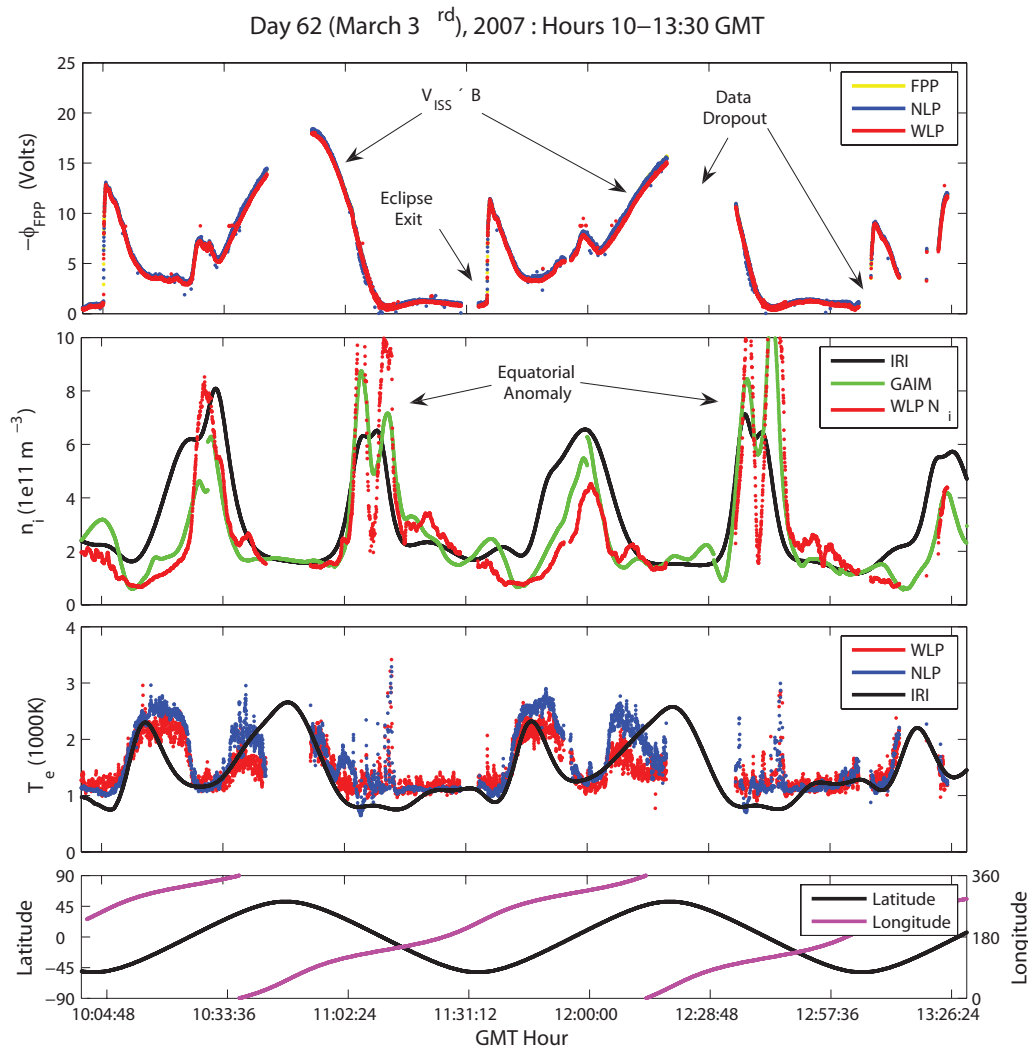
FIG. 12. (Color) The caption is the same as for Fig. 11.
