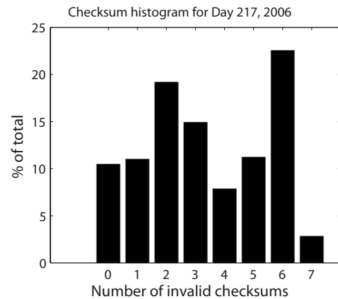
FIG. 2. Histogram of the number of invalid checksums when recalculated over the received page on the ground station. A value of 0 means all seven checksums were valid and the page was received uncorrupted.
