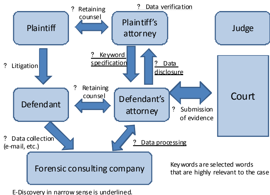
Figure 2. e-Discovery Procedure
