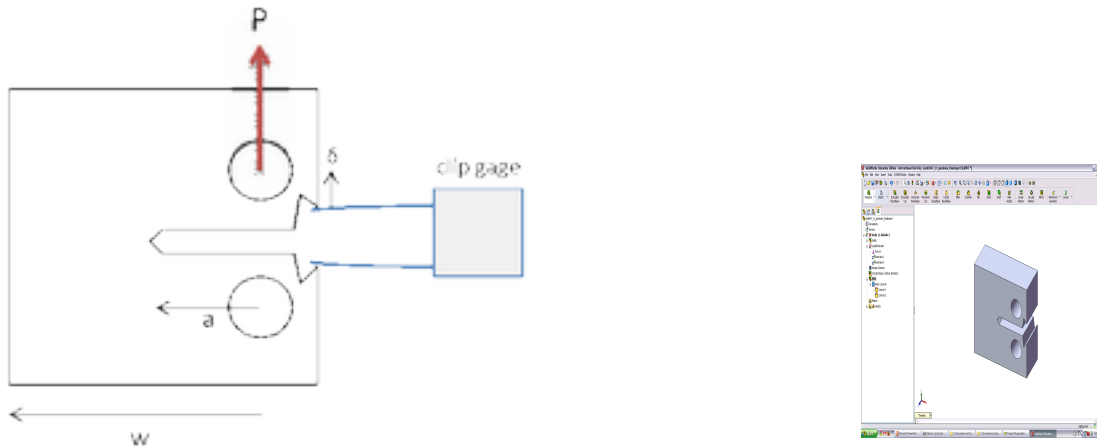
Figure 161618 - Model of compact tension specimen.
