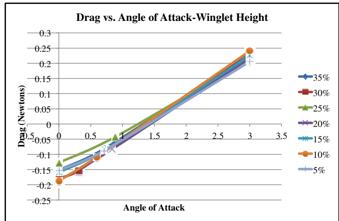
Figure 22. Drag vs. \alpha . Winglet Height
