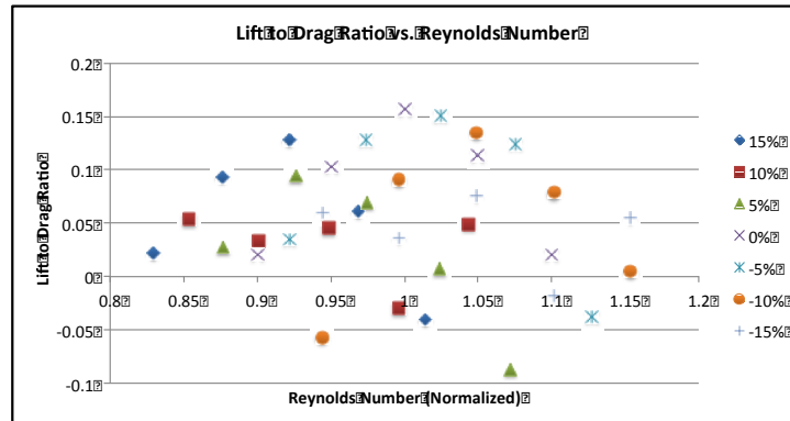
Figure 40. Lift to Drag Ratio vs. Reynolds Number. The graph clearly shows that the lift to drag ratio peaks at a Reynolds number of approximately 1 (normalized).
