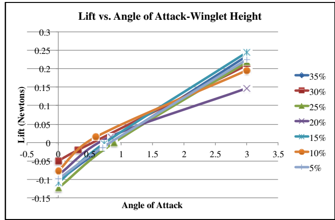
Figure 21. Lift vs. \alpha . Winglet Height
