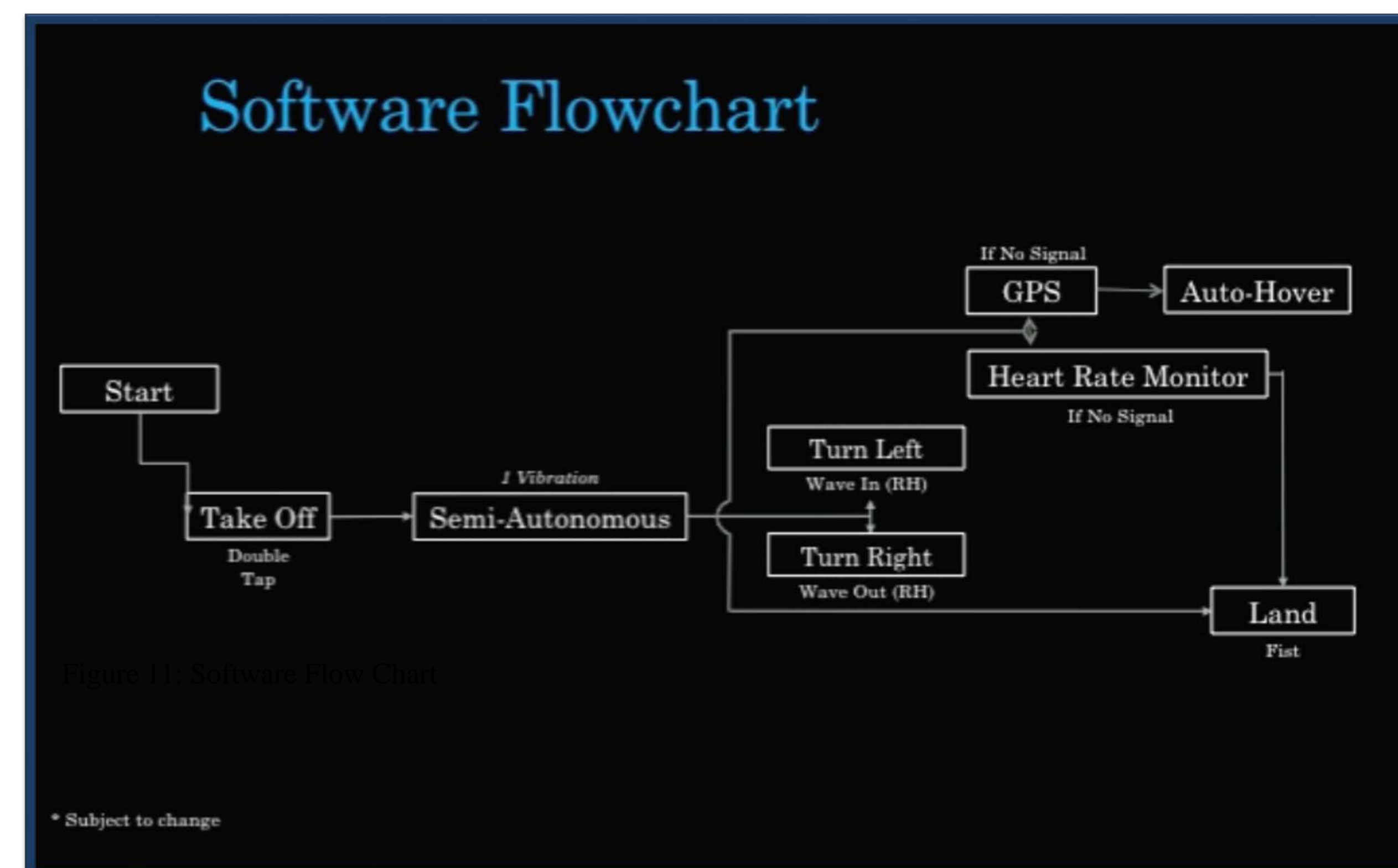
Figure 7: Code Logic
