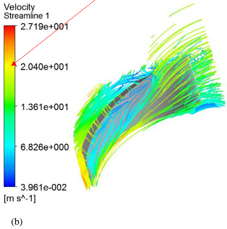
Figure 33: Streamline Distribution through the Impeller Blade (a, b)
