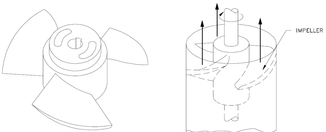
Figure 9: Axial Flow Pump
