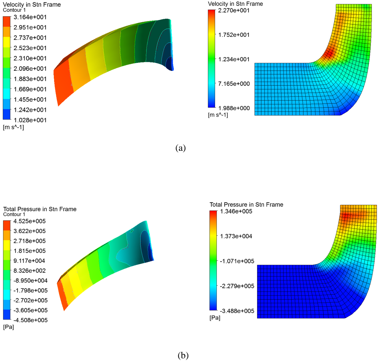
Figure 42: Optimized Min and Max Velocity and Pressure through the Impeller Blade (a, b)
