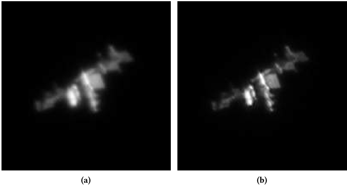
Figure 5.12: The International Space Station imaged on April 2, 2015 by the CDK20 and ML8050 in I band. The single 50 ms exposure (a) is significantly sharpened by applying a Van Cittert deconvolution (b).
