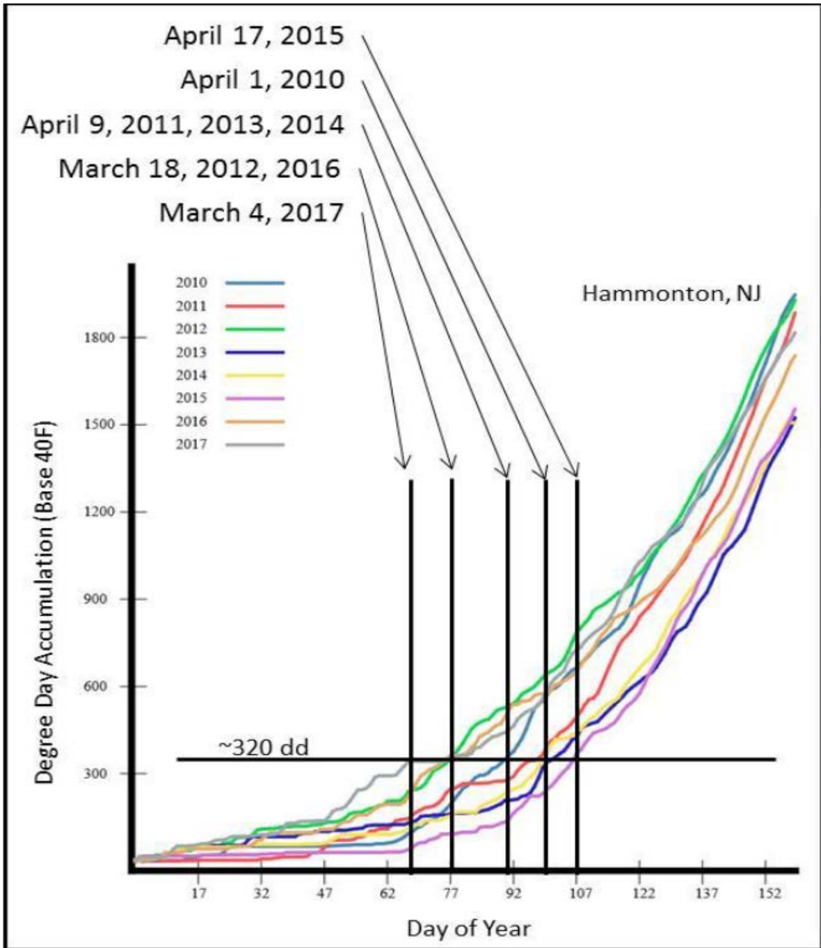
Fig. 1. Comparison of degree day accumulations for Hammonton, NJ taken from the degree day calculator ( http://benedick.rutgers.edu/Blueberryweather/ ).
