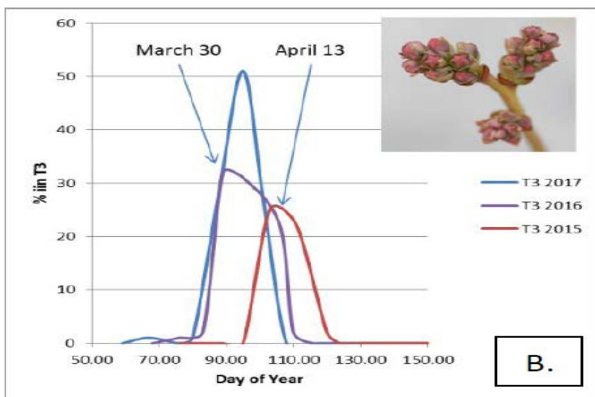
Fig. 2. A. Phenology of blueberry development (cv Duke) for 2017 in Hammonton NJ. B. Comparison of T3 budbreak for 2015-2017.
