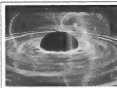
Black holes found in our Galaxy and at the center of quasars over the past three decades
