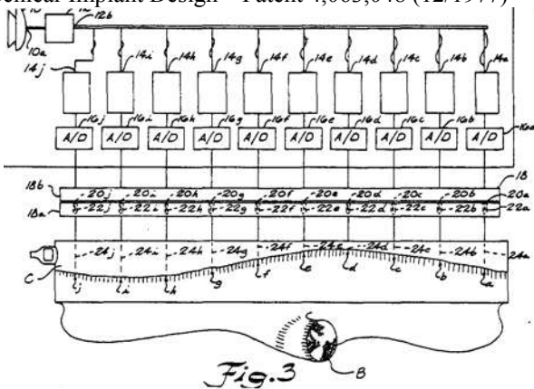
Cochlear Implant Design – Patent 4,063,048 (12/1977)
