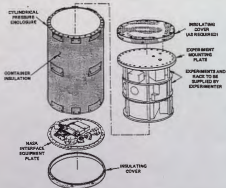
Figure-3: Get Away Special (GAS) Payload Accommodations
