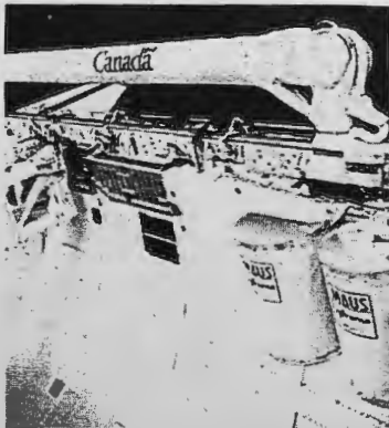
Figure-13: GAS Cans Mounted to Cargo Bay Sidewall
