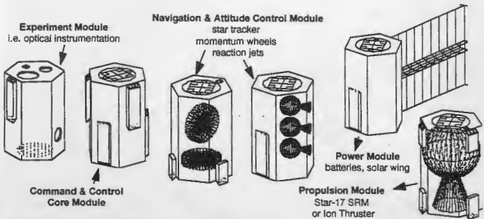
Figure-12: Deployable ISOBUS Module Building-Blocks
