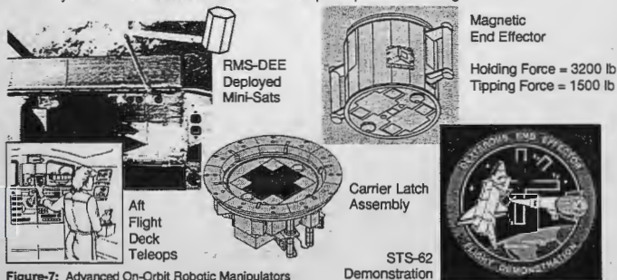
Figure-7: Advanced On-Orbit Robotic Manipulators and End-Effectors
