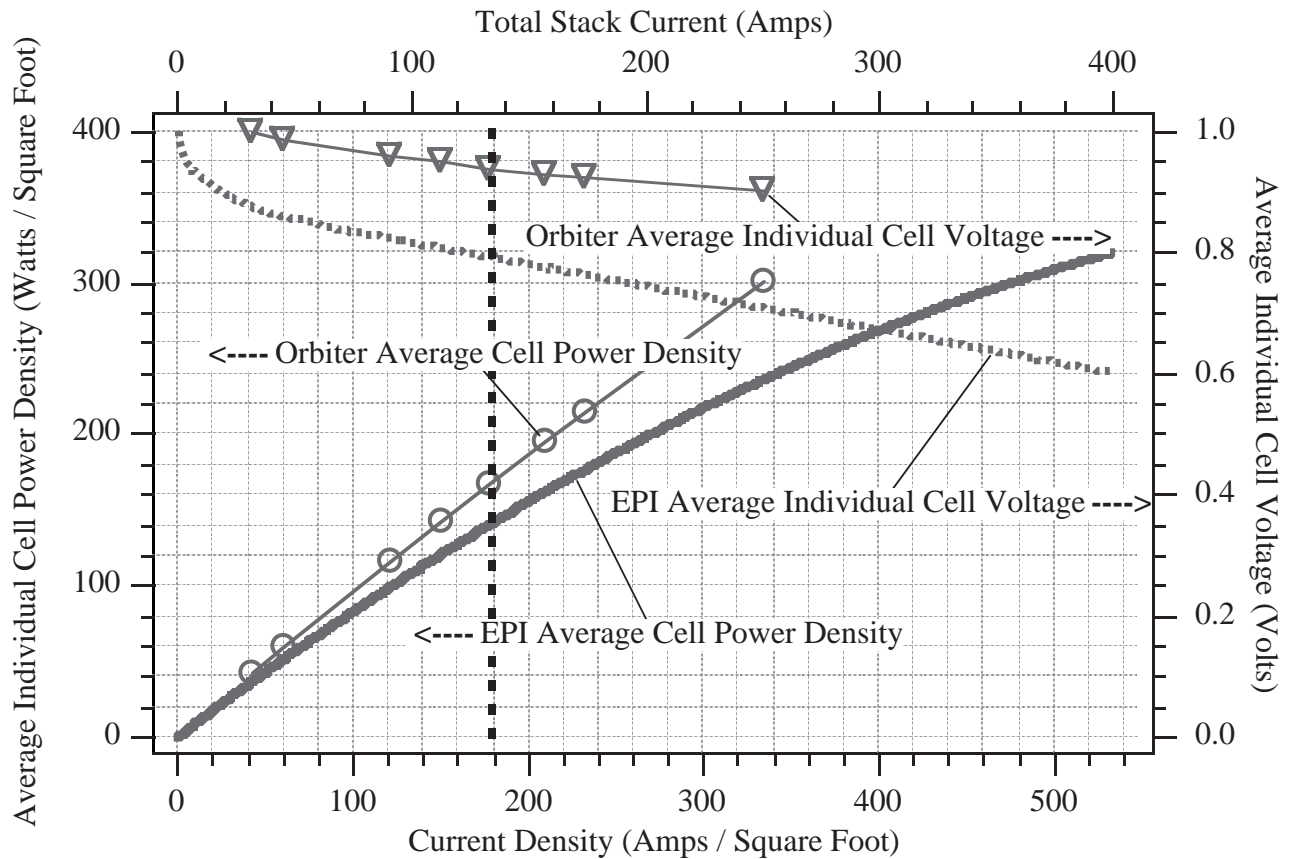
Figure 1. Average Cell Voltage and Average Cell Power Density vs. Total Stack Current and Cell Current Density for both the current Orbiter Alkaline Fuel Cell and the Energy Partners, Inc. Fuel Cell evaluated as part of the test program.
