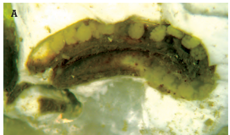
Figure 3 (A) Photo-micrograph (8x) showing a portion of an excavated burrow containing 15 separate egg cases. The female worm has been removed for clarity. P. Rawson photo. (B) A six-setiger (6 segment) swimming larva of P. websteri . P. Rawson photo.
