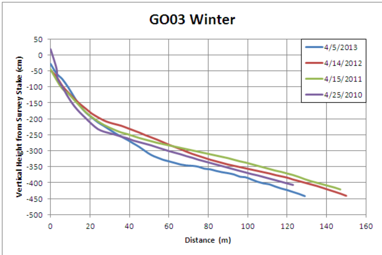
Figure 68. Winter beach profiles for GO03 from 2010, 2011, 2012, and 2013.
