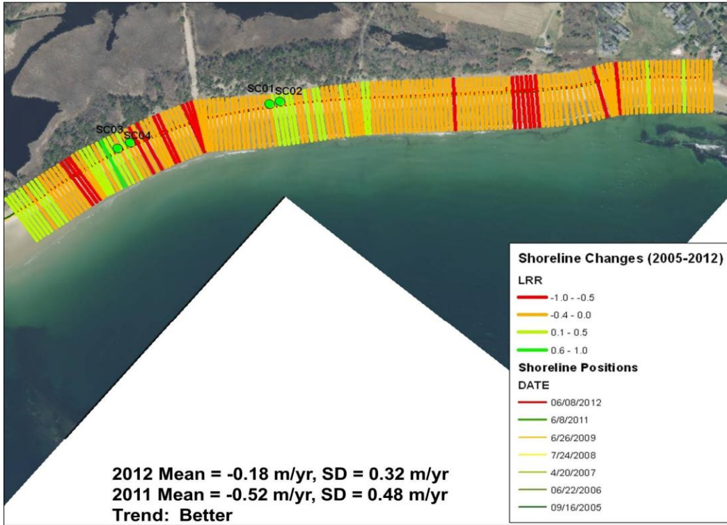
Figure 24. MBMAP results for Scarborough Beach. Base imagery from Maine OGIS.
