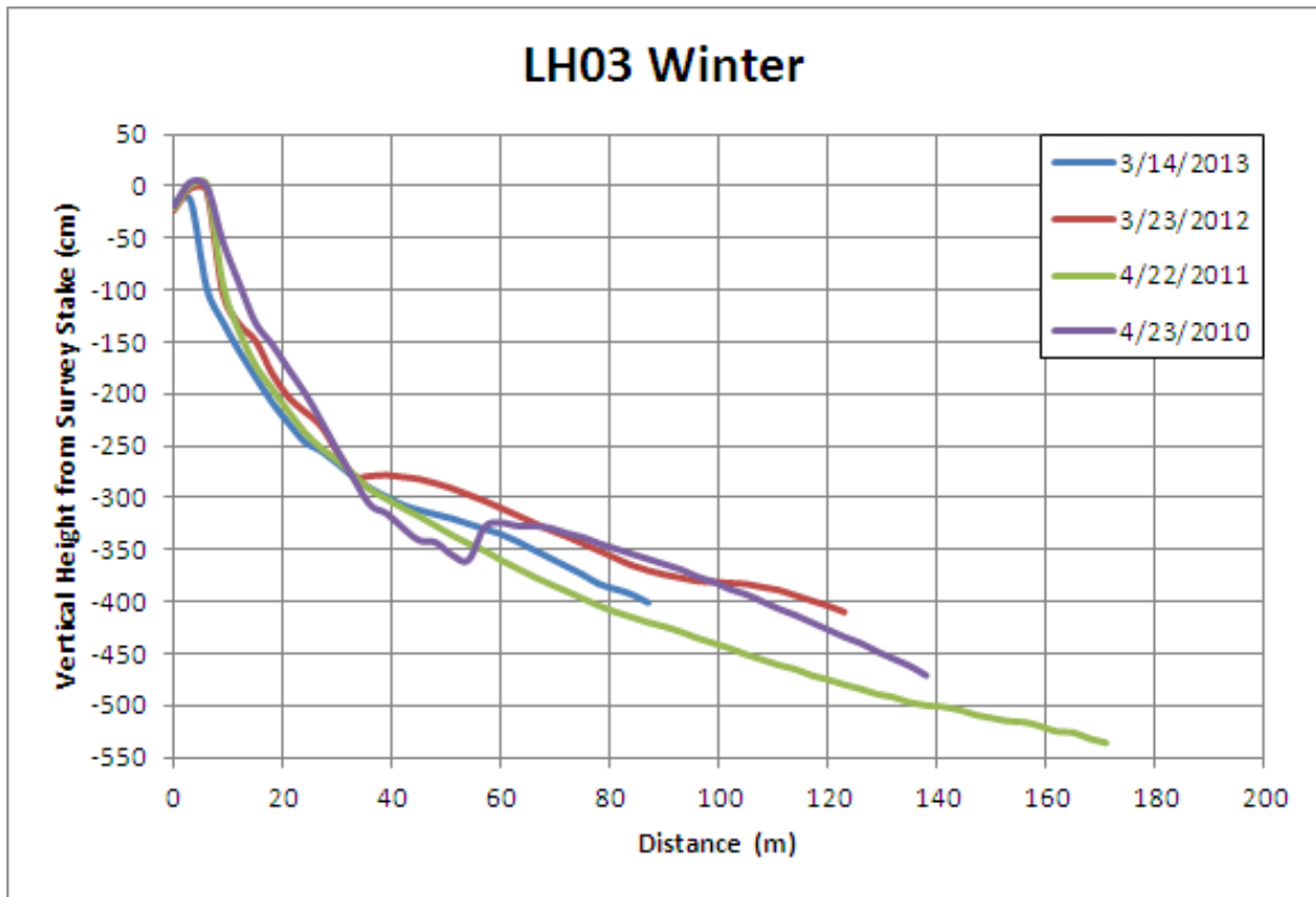
Figure 77. Winter beach profiles for LH03 from 2010, 2011, and 2012.
