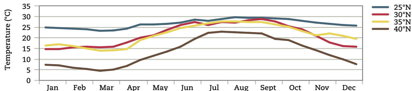
12. 2013 Seawater temperature profiles from NOAA coastal buoys at approximately 25, 30, 35 and 40 degree north latitudes. Based on mean bi-monthly data from NOAA buoys SMKF1-FL, 41112-FL, 41036-NC, 44065-NY. Data from ndbc.noaa.gov.
