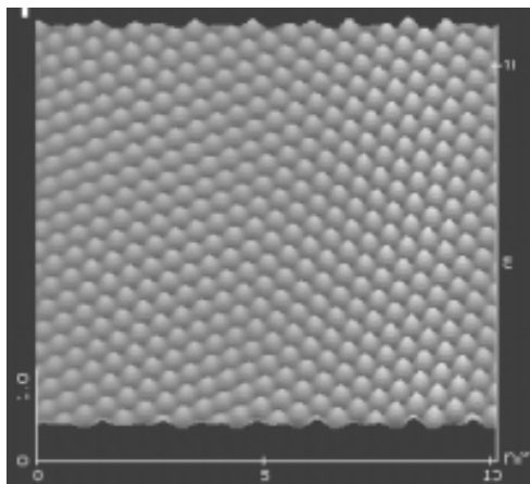
Figure1 (Mica , X & Y axes are 10nm)
