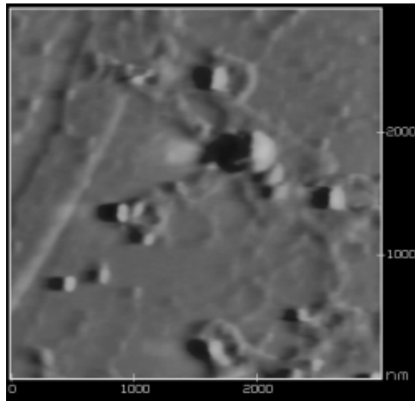
Figure 3 DNA on evaporated gold 3 micrometers on the X and Y axes. The tallest Z axis features are 46 nm Note the fine filamentary structures
