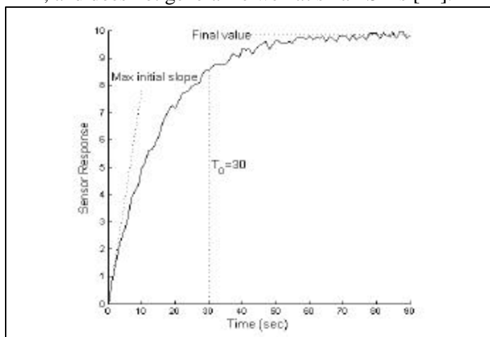
Figure 2 – Typical Time Response of a Single Sensor
