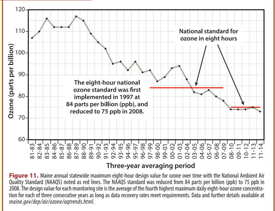
Ozone in Maine 1981–2014
