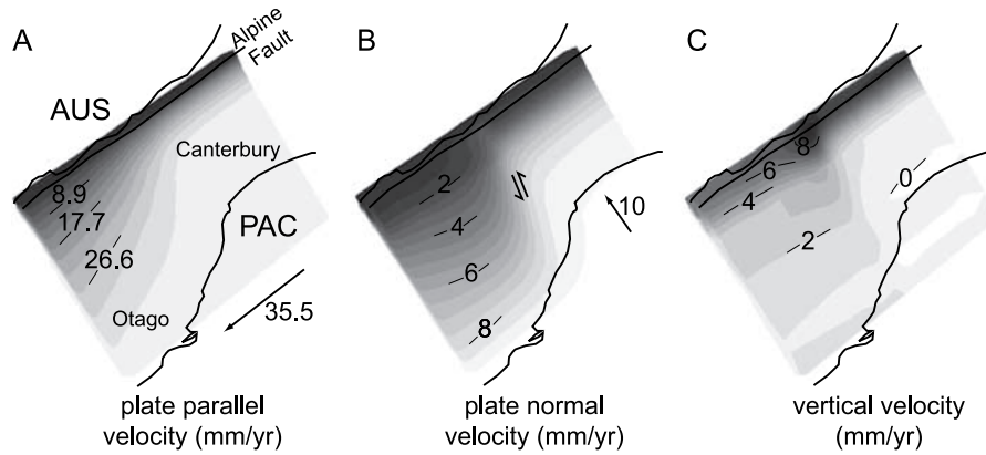
Figure 5. Model results overlain onto an outline of the South Island. (a) Contours of plate-parallel velocity relative to a fixed Pacific plate. (b) Contours of plate-normal velocity relative to a fixed Pacific plate. (c) Absolute uplift rate. See text for explanation.
