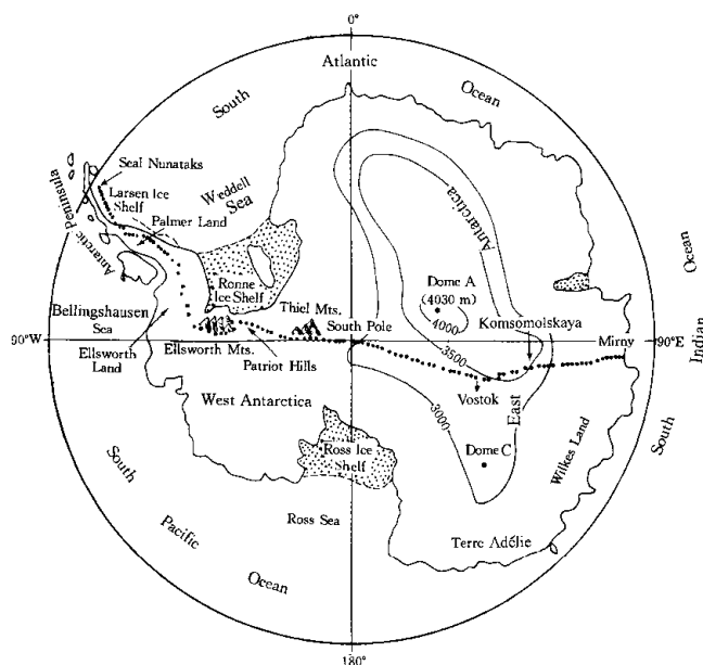
Fig. 1. Antarctic map showing the route of the 1990 ITAE and the sampling sites listed in Table 1.
