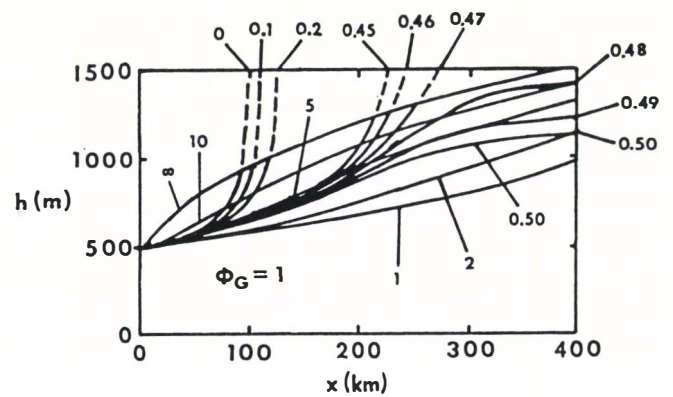
Fig. 12. The lengthening reach of a marine ice stream into an ice sheet during the inception and growth stages, shown as flowline profiles for various c values in Equation (58) when \phi_G = 1 specifies no ice-shelf buttressing. As c increases, the concave stream-flow profile (excluding dashed parts of surface-elevation curves) migrates toward the ice divide, with substantial down-draw of sheet flow occurring after a surface-inflection instability at 0.47 < c < 0.48 . Stream flow steadily reverts to sheet flow for c > 1 , causing the flowline elevation to increase and its profile to become increasingly convex.
