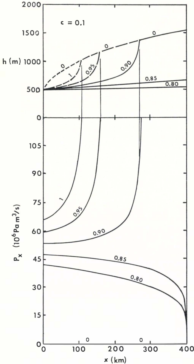
Fig. 15. Pulling power during the life cycle of an ice stream emphasizing the inception stage, with c = 0.1 and \phi_G decreasing from unity to zero. As the ice stream retreats without concomitant down-draw of the ice sheet (top), pulling power is concentrated at the head of the ice stream (bottom). After down-draw begins for \phi_G < 0.90 (top), pulling power becomes greatest toward the foot of the ice stream (bottom).
