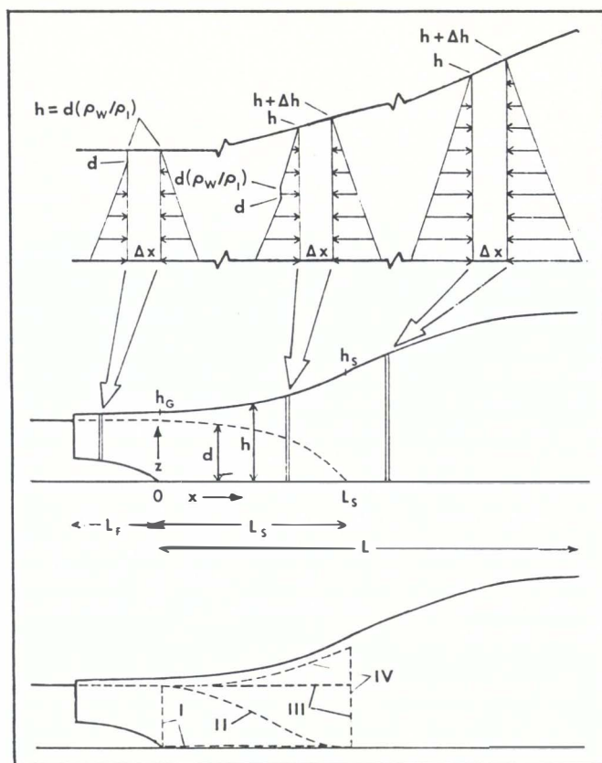
Fig. 3. Pulling forces defined as net horizontal lithostatic and hydrostatic forces acting in a marine flow band of an ice sheet. Horizontal lithostatic and hydrostatic forces pressing against imaginary ice columns are shown for sheet flow (right), stream flow (center) and shelf flow (left), with the flow band having floating length L_F , grounded length L and streaming length L_S .
