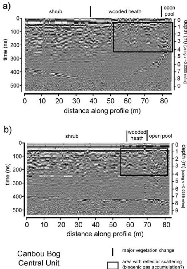
Figure 3. GPR profile results along (a) line c2 and (b) line c3 (see Figure 1b for location) in the Central Unit of Caribou Bog. Vegetation at surface, open pools, and well location are also shown. Squares outline areas showing GPR reflector scattering interpreted as free-phase biogenic gas accumulations.
