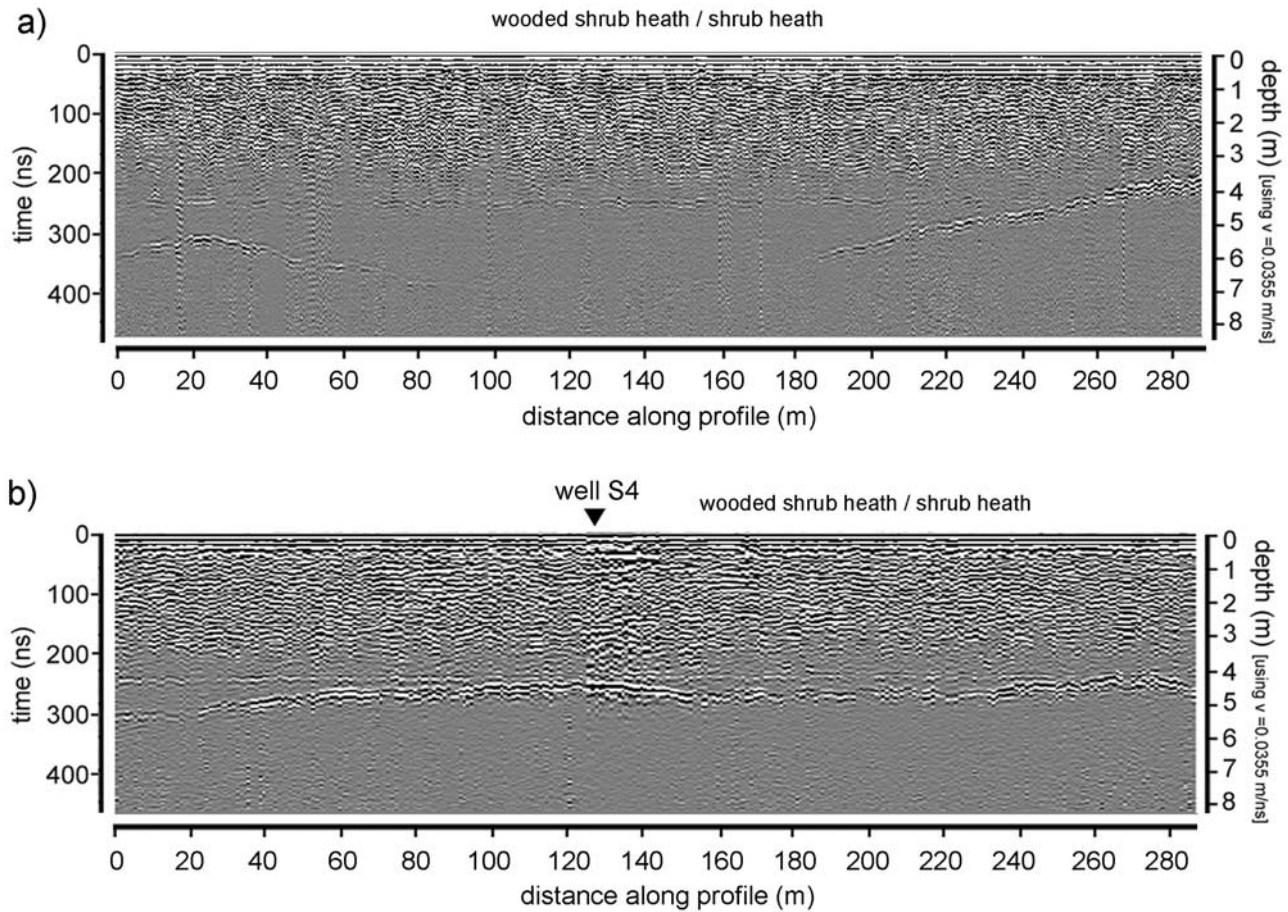
Figure 5. GPR profile results along (a) line s2 and (b) line s3 (see Figure 1c for location) in the Southern Unit of Caribou Bog. Vegetation at surface and well locations are also shown.
