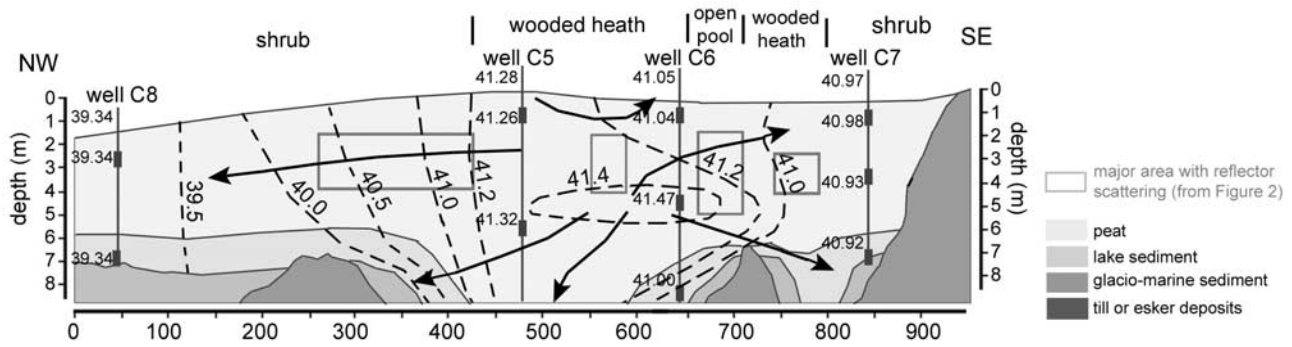
Figure 7. Interpreted cross section of the Central Unit of Caribou Bog (line c1) showing the hydraulic head values as a function of depth, and the interpreted groundwater flow directions during April 2000. Major vegetation patterns and the location of pools at the surface are also shown. GPR data and core measurements are used to define the lake sediment-mineral soil interface.
