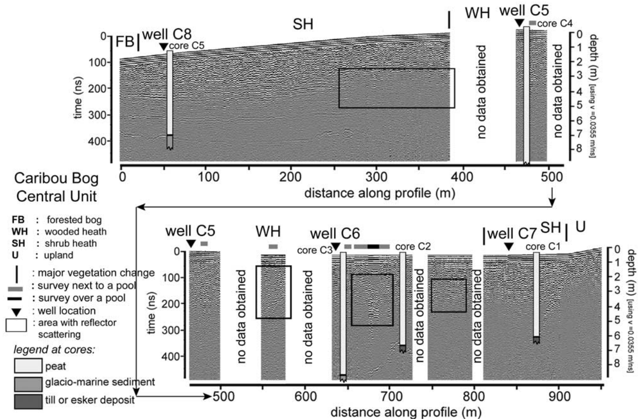
Figure 2. GPR profile results along line c1 (see Figure 1b for location) in the Central Unit of Caribou Bog. Vegetation at surface, open pools, well location, and coring results are also shown.
