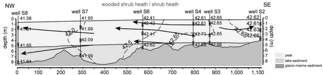
Figure 6. Interpreted cross section of the Southern Unit of Caribou Bog (line s1) showing the hydraulic head values as a function of depth, and the interpreted groundwater flow movement during May 2000. Major vegetation at surface is also shown. GPR data and core measurements are used to define the lake sediment-mineral soil interface.
