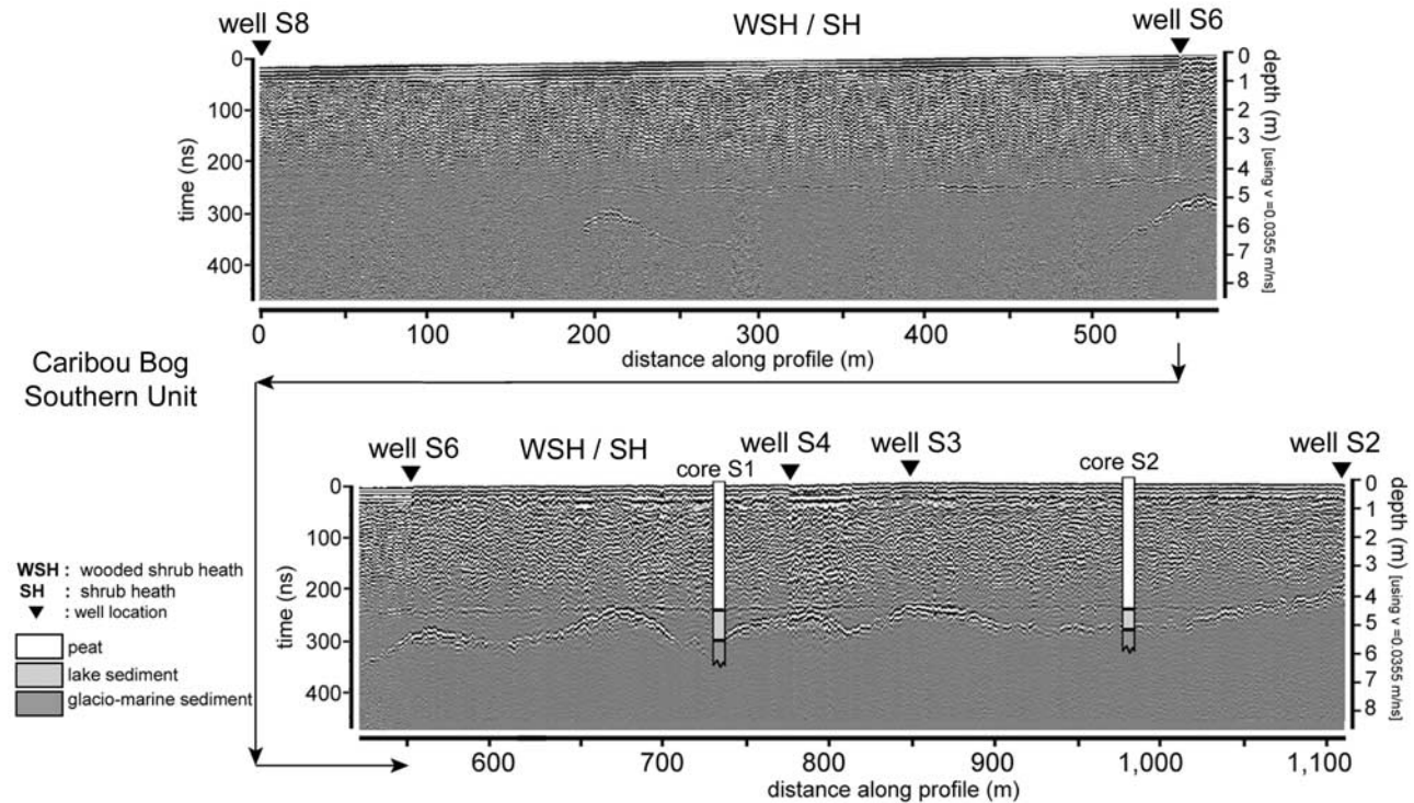
Figure 4. GPR profile results along line s1 (see Figure 1c for location) in the Southern Unit of Caribou Bog. Vegetation at surface, well location, and coring results are also shown.
