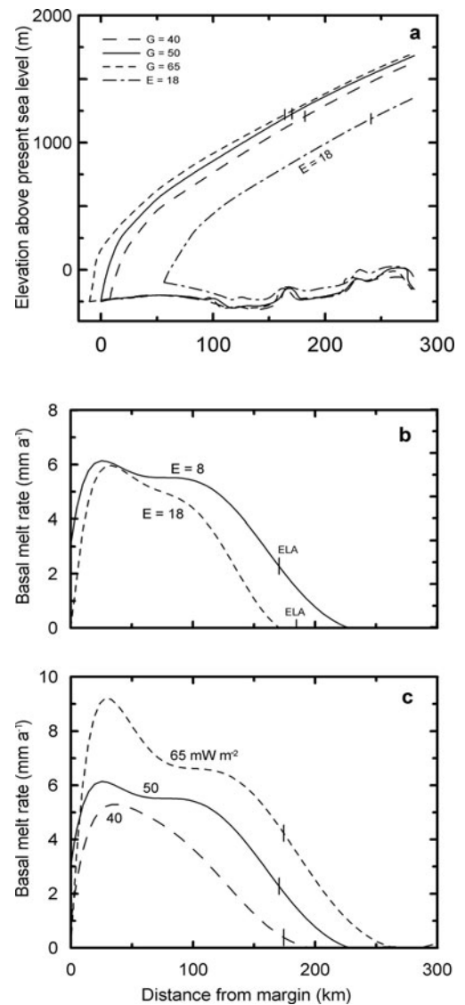
Fig. 8. Sensitivity tests: (a) effect of geothermal flux and enhancement factor on surface profile at 15.6 ka; (b) effect of enhancement factor on basal melt rate at 15.6 ka; and (c) effect of geothermal flux on basal melt rate at 15.6 ka. Tick marks show locations of equilibrium lines.
