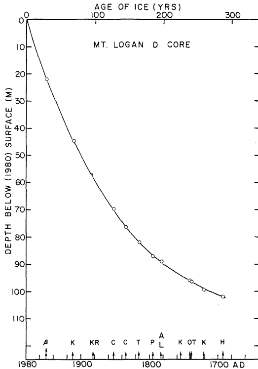
FIG. 2 Depth vs time scale plot for the Mt. Logan core. Volcanic events identified through the chemical signatures are marked by vertical arrows. The double arrow marks the end of the \beta -activity dating.
