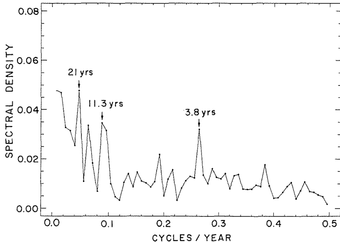
FIG. 5 Fourier transform power spectrum of Mt. Logan net accumulation time series from AD 1736–1985. Physically significant spectral peaks are marked.
