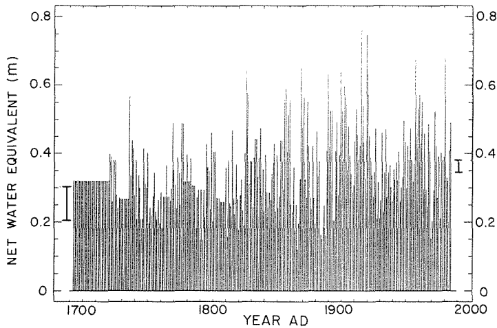
FIG. 4 Mt. Logan net accumulation time series (metres water equivalent): AD 1693–1985.
