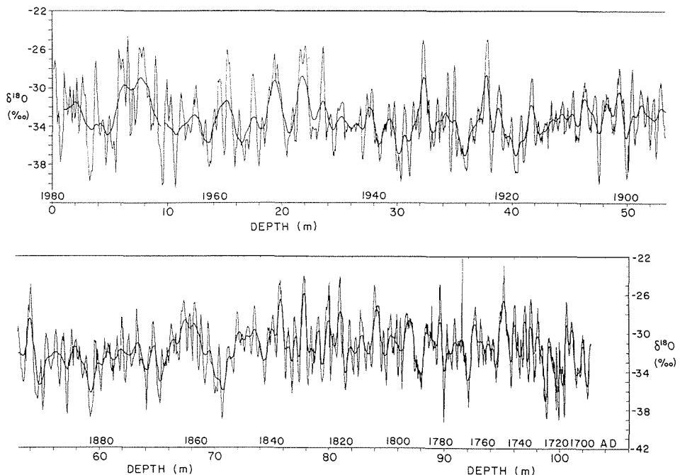
FIG. 1 \delta^{18}\text{O} (‰) vs depth in the core. Nonlinear time scale is marked above the depth scale.
