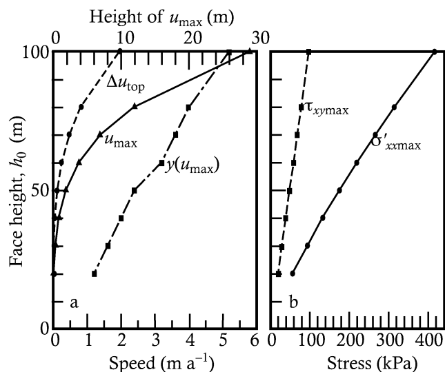
Fig. 6. Variation of velocity and stress indices with face height for water-free, zero basal velocity simulations listed in Table 2. (a) Speeds, including u_{\max} and \Delta u_{\text{top}} along with the height at which u_{\max} occurs on the face, read against the upper axis. (b) Maximum values of \sigma'_{xx} and \tau_{xy} in the flowplane.
