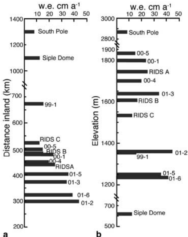
Fig. 4. Accumulation rates vs (a) distance inland (km), and (b) elevation (m).
