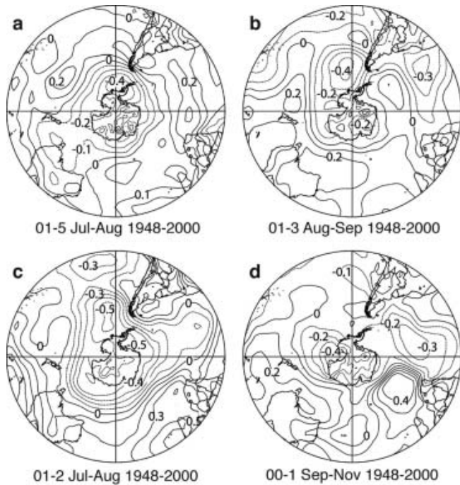
Fig. 8. Correlations of the annual accumulation-rate records from sites 01-5 (a), 01-3 (b), 01-2 (c) and 00-1 (d) and SLP from the NCEP re-analysis. Images created on the US National Oceanic and Atmospheric Administration (NOAA)–Cooperative Institute for Research in Environmental Sciences (CIRES) Climate Diagnostics Center web site at http://www.cdc.noaa.gov/ .
