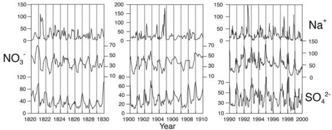
Fig. 3. Annual chemistry layers ( \mu\text{g L}^{-1} ) from the 00-1 ice core used for dating. Detailed 10 year sections (1820–30, 1900–10, 1990–2000) display winter–spring ( \text{Na}^+ ) and summer ( \text{NO}_3^- , \text{SO}_4^{2-} ) maxima. Clear seasonal signals are present in all records.
