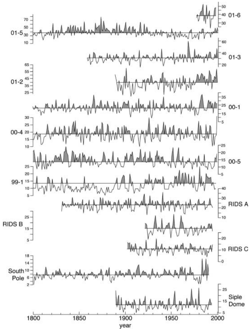
Fig. 1. The 13 annual accumulation-rate records in w.e. ( \text{cm a}^{-1} ), 1800–2001. The line through each record denotes the mean for the full record, and the shading indicates accumulation above the mean.
