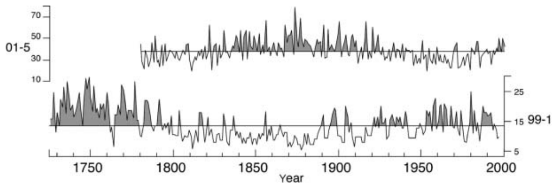
Fig. 5. Accumulation-rate records in \text{cm a}^{-1} w.e. for the full record for sites 01-5 and 99-1. The line through the record denotes the mean accumulation, and the shaded portions of the record are above mean accumulation. The trends may be due to topographical effects.
