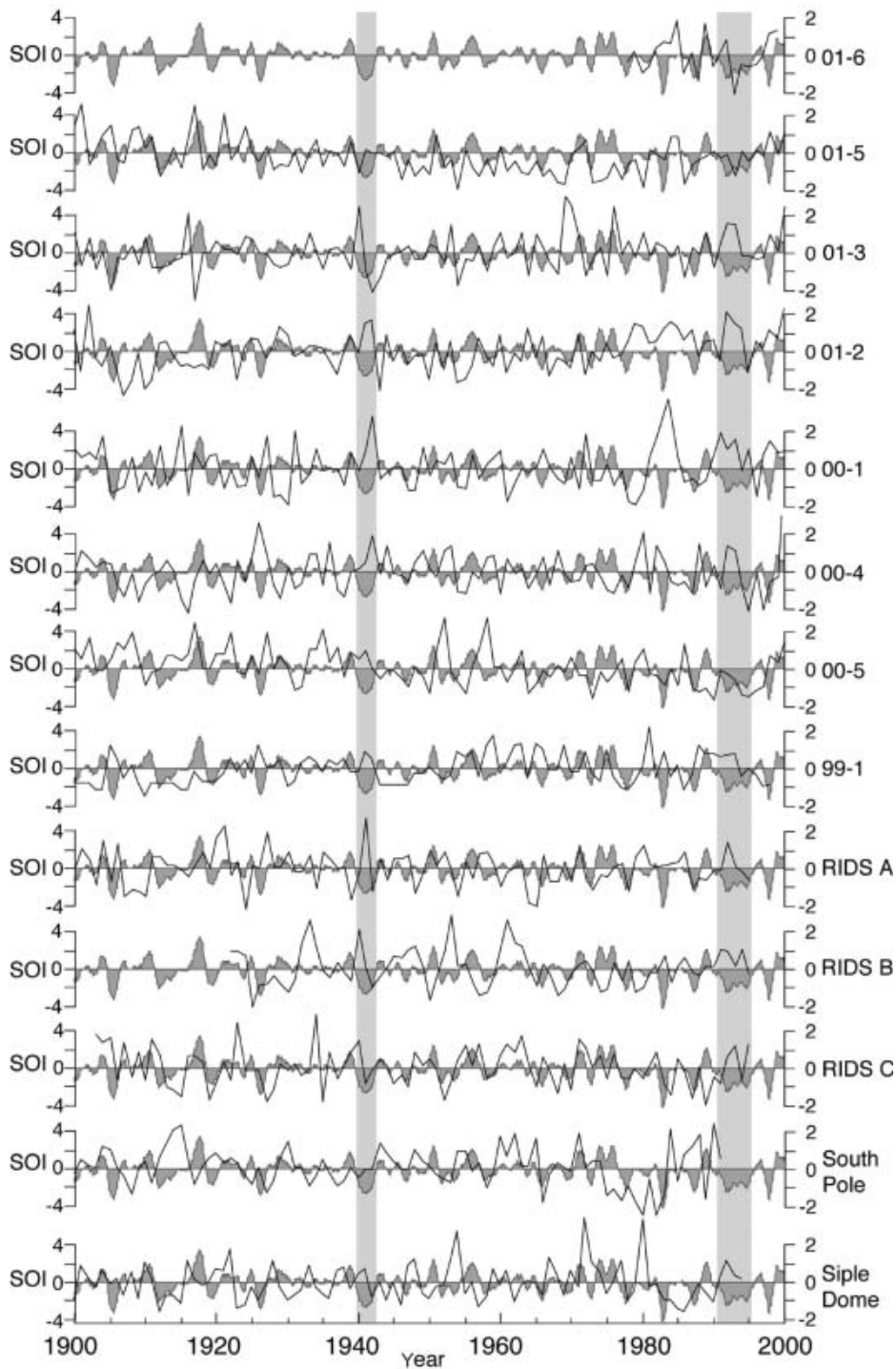
Fig. 7. The normalized (anomaly from the mean divided by the standard deviation) accumulation-rate records (black line) and the SOI (shaded grey) smoothed with a 12-point running mean, from 1900 to 2000. The highlighted periods 1940–42 and 1991–95 indicate above-mean accumulation during the two most sustained periods of negative SOI during the 100 year record.
