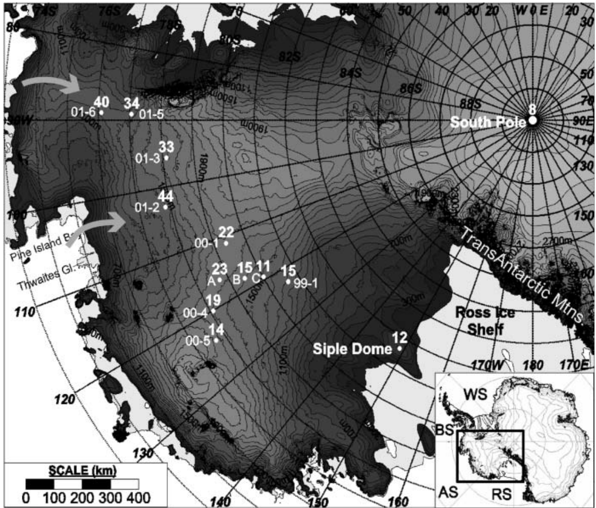
Fig. 2. Ice-core locations and mean accumulation rates, 1922–91. Core site locations: 01-06, 01-5, 01-3 and 01-2 in the Pine Island–Thwaites drainage system; 00-1, RIDS A, 00-4 and 00-5 near the ice divide; and RIDS B, RIDS C, 99-1 and Siple Dome in the Ross drainage system. The arrows indicate dominant moisture pathways. WS, Weddell Sea; BS, Bellingshausen Sea; AS, Amundsen Sea; RS, Ross Sea; A, RIDS A; B, RIDS B; C, RIDS C. A digital elevation model was used to produce the shaded relief map (Liu and others, 2001).
