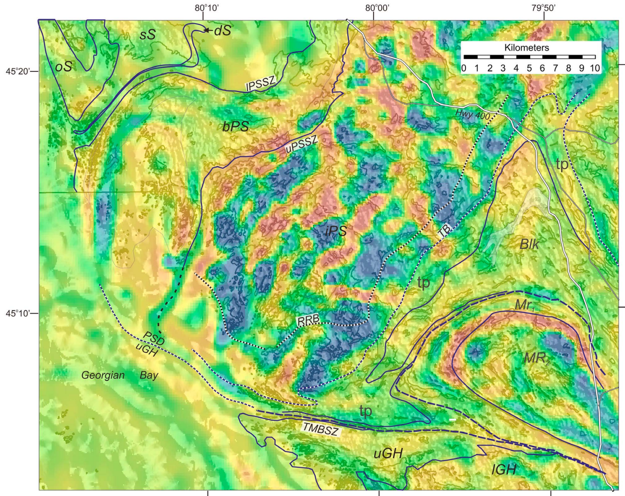
Figure 4. First vertical derivative of total magnetic field [Canadian Aeromagnetic Data Base, 2008] draped on topography and bathymetry (courtesy of U. S. NOAA, National Geophysical Data Center) for southwest end of Parry Sound domain and parts of contiguous domains between Highway 400 and Georgian Bay. Key for first vertical derivative magnetic map: dark blue to green, 0.212–0.023 nT/m; light green to yellow, 0.024 to -0.045 nT/m; yellow to red, -0.046 to -0.186 nT/m. Unit boundaries as in Figure 2. The Parry Sound domain–uGH boundary (coarse dashed blue line; lower boundary of tp in west) is projected along bathymetric ridges and magnetic anomalies; a second dashed line indicates projection of uPSSZ.
