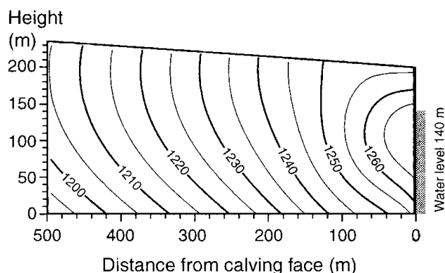
Fig. 3. Contours of horizontal velocity, u_i , in the last 500 m of a glacier 200 m thick at the calving face. S_f = 0.5 for this simulation. Contour interval is 5 m a^{-1} .
