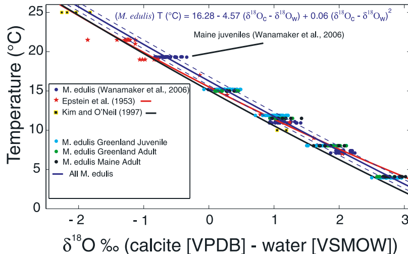
Figure 4. Paleotemperature relationships from this study (turquoise circles, Greenland juveniles; green circles, Greenland adults; black circles, Maine adults) (solid blue line is equation (4); dashed blue lines are upper and lower error of 0.57^{\circ}\text{C} ), Wanamaker et al. [2006] (blue circles; equation (3)), Epstein et al. [1953] (red stars and red line; equation (1)) and Kim and O'Neil [1997] (black and yellow squares and solid black line; equation (2)).
