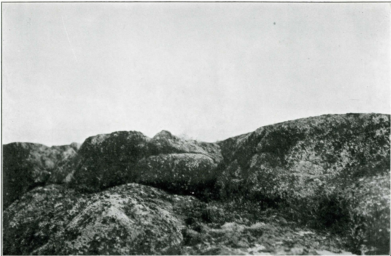
GLACIATED SUMMIT OF SARGENT MOUNTAIN, MOUNT DESERT. FIG. 6.
