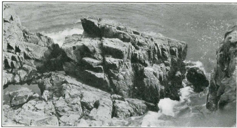
JOINT CONTROL OF SEA EROSION. FIG. 8.
