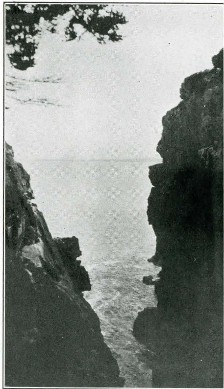
CHASM DUE TO SEA EROSION. At Otter Cliffs. FIG. 9.
