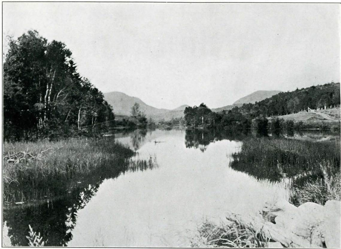
FIG. 14. LONG POND: LAGOON ENCLOSED BY BAR.
