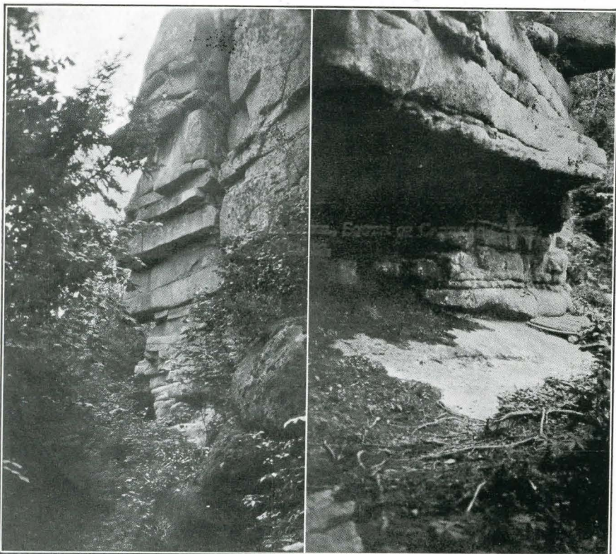
CADILLAC CLIFFS, GORHAM MOUNTAIN. FIG. 10.
