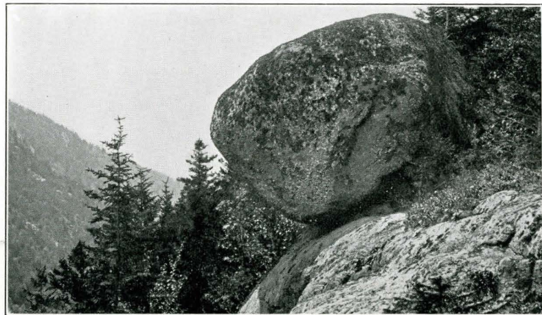
BALANCED ROCK, SOUTH BUBBLE, MOUNT DESERT. FIG. 2.
