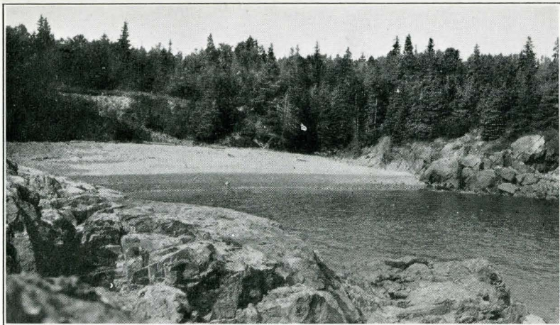
HUNTER BEACH COVE, SOUTH SIDE MOUNT DESERT. Breccia on left. FIG. 1.
