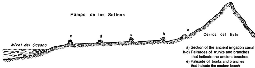
Figure 3. REY Y BASADRE's (1896) diagram of Santa beach ridges showing palisades of driftwood on all ridges.
