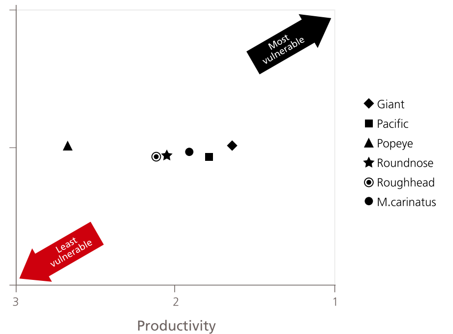
Figure 10. Results of the PSA analysis using productivity scaled only to grenadier species (global scale, not fisheries specific, see Table 1 for data and Table 3 for attributes) and susceptibility attributes and scaling of Cope et al. (in press). An ad hoc Working Group Analysis of the PSA Method
