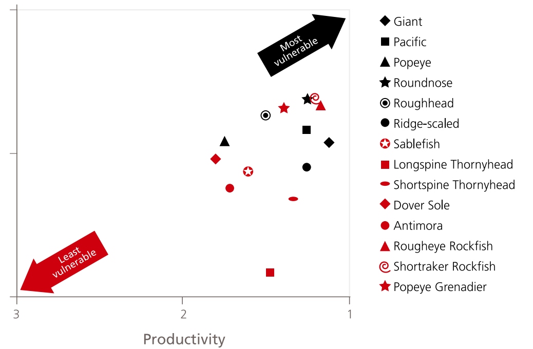
Figure 9. Results of the PSA analysis using the attributes and scaling of Cope et al. (in press), see Table 2 for attributes. All grenadier species (globally) are illustrated with black symbols and red symbols are shelf and slope species of the North Pacific (off the California coast).
