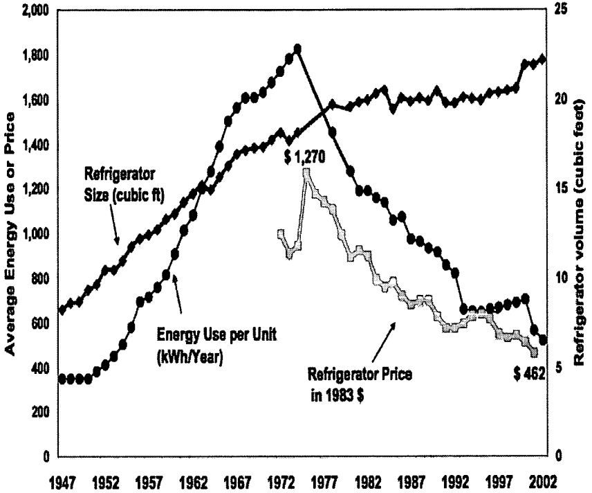
Figure 8 - New U.S. refrigerators: average annual energy use and retail prices, 1947-2002. 381
