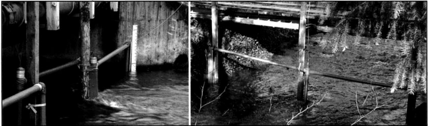
Photo 1. PIT tag interrogation systems on Abernathy Creek, Longview, WA, (Left panel: AB-UP and right panel: AB-DN). Arrays at both sites consisted of multiple antennas oriented such that they spanned the width of the stream channel.
