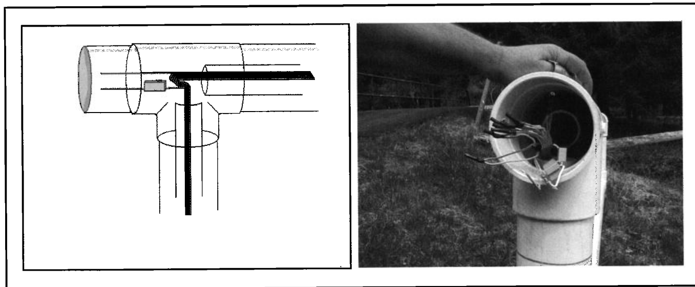
Figure 3. Schematic of antenna construction and photograph of antenna coil in PVC pipe. Antenna wires were fed through the smaller diameter PVC pipe (5.1 cm) centered within a larger diameter PVC pipe (10.2 cm). Wires were not overlapped or twisted when feeding the coil through the PVC pipe.
