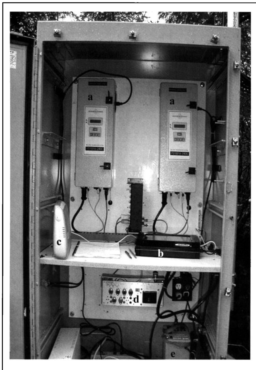
Photo 3. PIT tag transceiver (a), computer (b), satellite modem (c), AC/DC converter (d), and isolation transformer (e) used on Abernathy Creek, Longview, WA, AB-DN; each antenna was connected to one transceiver (note black cable in the bottom left corner of each transceiver).
