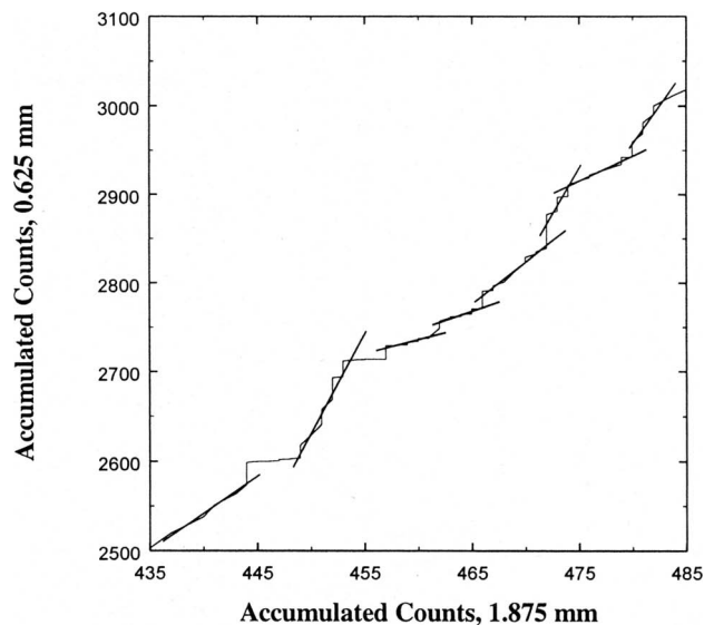
FIG. 7. Similar to Fig. 6 except that the counts correspond to video disdrometer “measurements” in a Monte Carlo simulation of statistically homogeneous rain as described in Jameson and Kostinski (1999). Drop size distribution patches are clearly identifiable.
