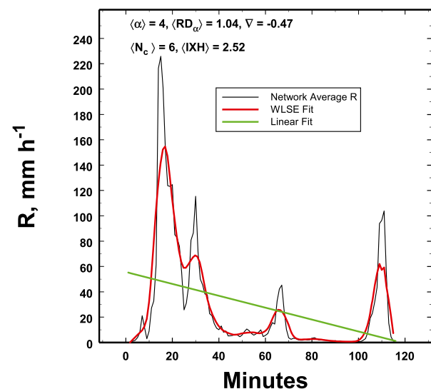
FIG. 4. The first approximately 120 min of the data in Fig. 3 for the convective rain in which the data are statistically heterogeneous.
