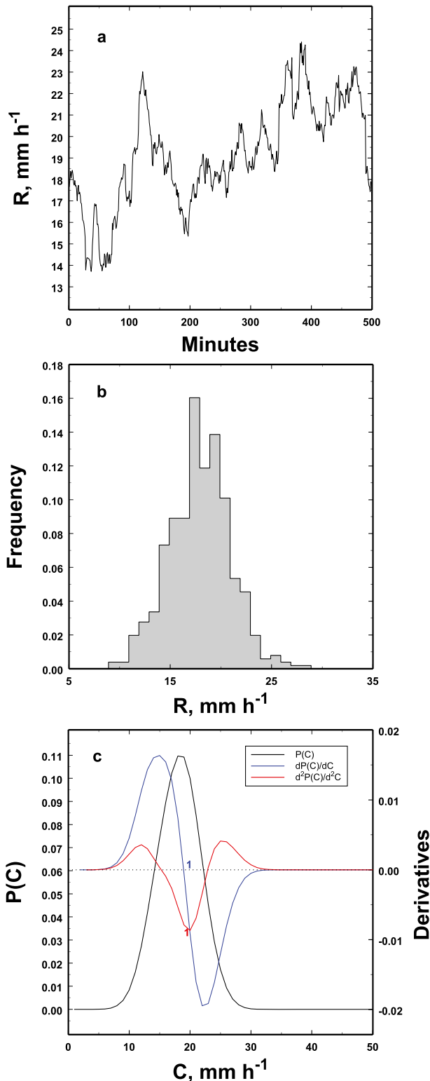
FIG. A1. (a) The time series plot of statistically homogeneous correlated rainfall rate shows no particular average value. (b) The frequency histogram for the data plotted in (a), suggesting one or two peak values. (c) The Bayesian inversion (black) distribution
