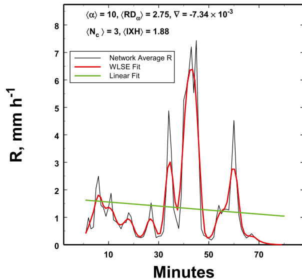
FIG. 7. As in Fig. 6, this is an 80-min mixture of different rain intensities on 26 Dec 2013, but unlike Fig. 6, this rain is statistically heterogeneous.
