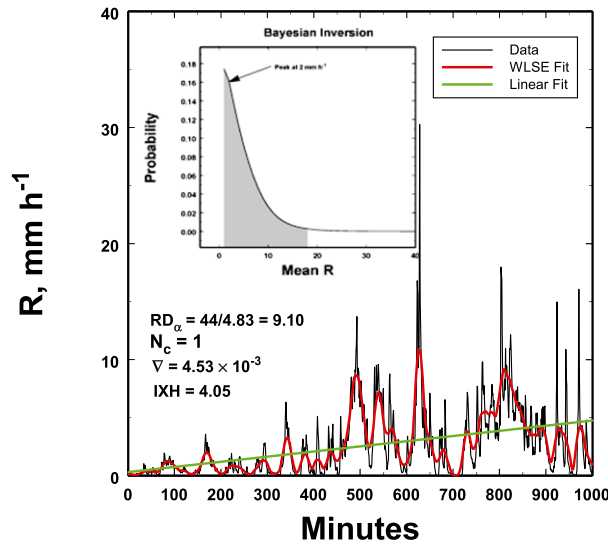
FIG. 2. Observations of rain in South Carolina. Despite there being only one Bayesian component, these data show significant statistical heterogeneity because of the increasing variance in time. The shading in the inset represents 99% of the distribution of the global mean values inferred from the Bayesian inversion. The term R has units of \text{mm h}^{-1} , and \nabla is the gradient of the linear fit across the data (green).
