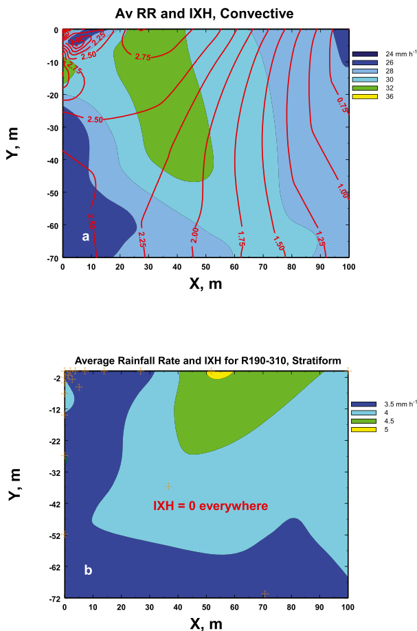
FIG. 10. (a) The 2D interpolated fields of the temporal average rainfall rate and IXH (red lines) for the convective rain during the 440-min rain event using each of the values of each instrument (orange crosses) separately. Clearly, depending upon location, there is significant variability in both the global mean rainfall rate and IXH, although all values of IXH are consistent with statistical heterogeneity. (b) The 2D interpolated fields of the temporal global mean rainfall rate and IXH for the stratiform rain during the 440-min rain event. The spatial variability is less than in (a), and the values of IXH over the entire area are consistent with statistical homogeneity.
