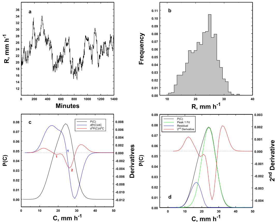
FIG. A3. (a) As in Fig. A2, but the two peaks are not so obvious in (b) the histogram. (c) However, while the first derivative detects only one component, the second derivative is still able to capture the presence of both components. (d) When the second derivative is indecisive, one can also resort to the technique of residuals, where the subtraction of one peak (green) from P(C) leaves a residual peak (blue) that is consistent with the second derivative (red). At some point all techniques might fail, but then the data are likely effectively statistically homogeneous anyway.
