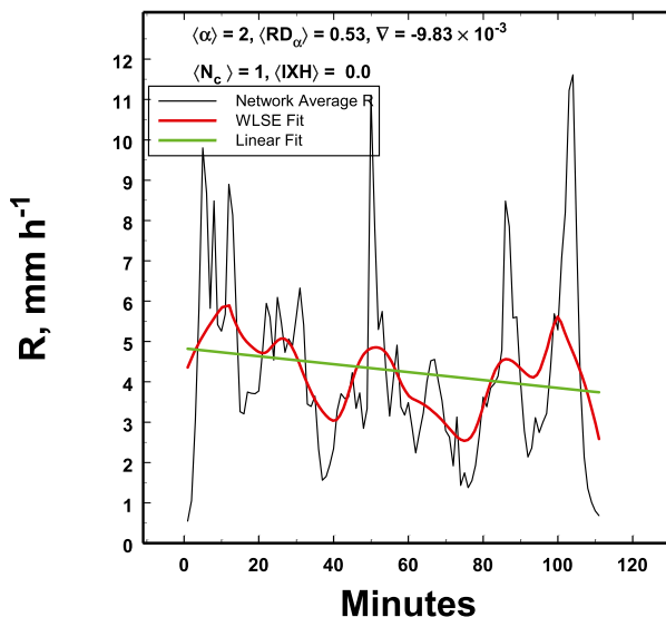
FIG. 6. The mixed period of rain (~200–300 min) in the 440-min rain event when background rain has occasional convective rain elements moving through, giving the appearance of being statistically heterogeneous. Despite this, the data are also statistically homogeneous as discussed in the text.
