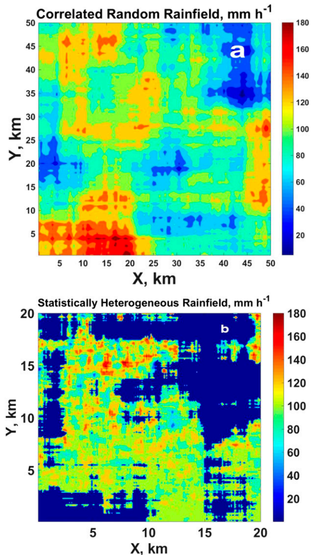
FIG. 12. Synthesized 2D rain fields (a) of a WSS rain field having \alpha = 0 and N_c = 1 so that IXH = 0 and (b) of a statistically heterogeneous rain field having \alpha = 14 , RD_\alpha = 2.03 , and N_c = 2 so that IXH = 0.77 , which is in agreement with the assumed inputs in both cases.
