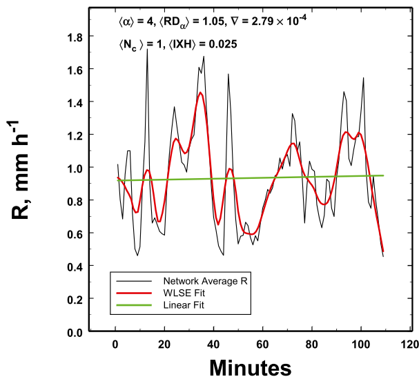
FIG. 5. Analysis of the stratiform period of rain during the 440-min rain event shows that it is statistically homogeneous as confirmed by the analyses of the global mean and fluctuating components as discussed in the text.
