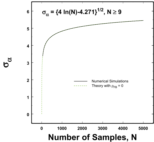
FIG. 1. The relation between the standard deviation \sigma_\alpha of \alpha to N observations determined from theory and confirmed using numerical simulations. The various lines are explained in the text, but the equation is used in the subsequent analyses.
