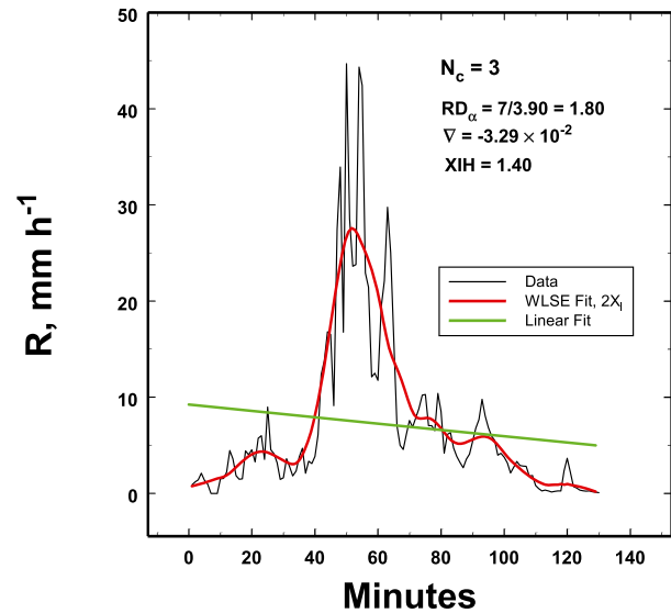
FIG. 8. Data from the NASA Wallops Island rain facility through a convective rainband passage preceding a warm front. These data are clearly statistically heterogeneous as discussed in the text.
