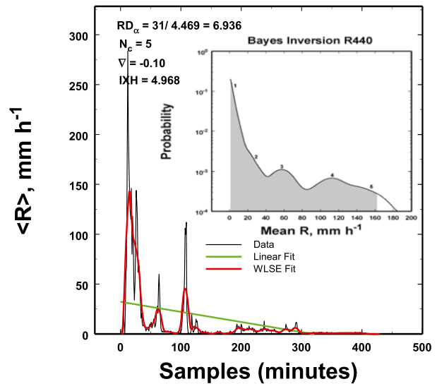
FIG. 3. The average values over a small network of 19 video disdrometers of a convective–stratiform rain event lasting 440 min as described further in the text. These data as a whole are statistically heterogeneous, but they can be divided into a statistically homogeneous section and a statistically heterogeneous section as presented next.
