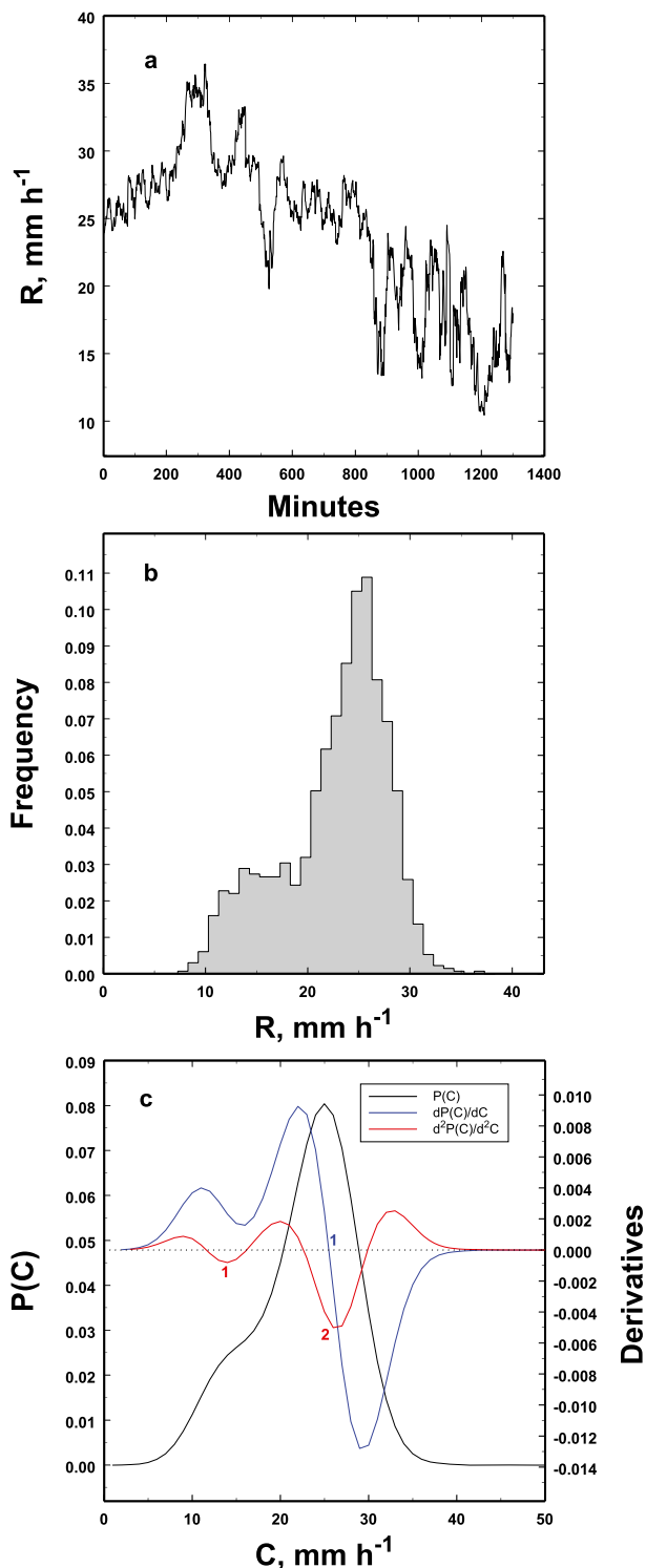
FIG. A2. As in Fig. A1, but for (a) a two-component statistically heterogeneous set of values. (b) The histogram clearly shows that there are likely two components. (c) However, the first derivative indicates only one component, but the second derivative detects the presence of both components, thus illustrating the importance of looking at the second derivative as well as the first derivative.
