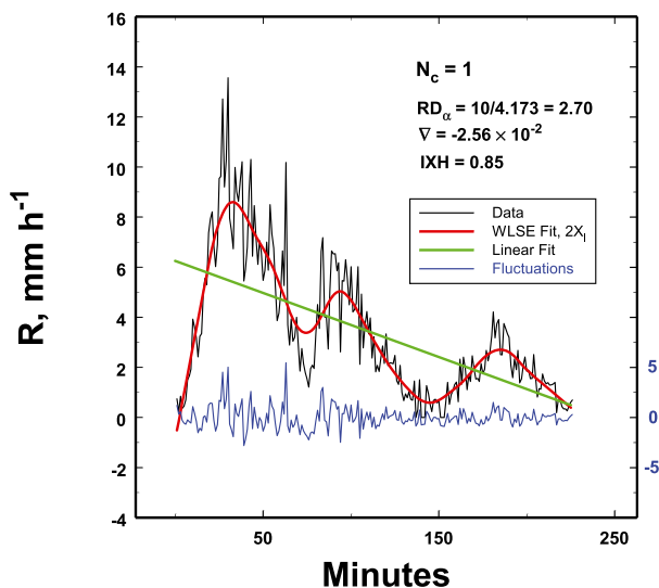
FIG. 9. A second set of data from Wallops Island is shown. The data are statistically heterogeneous because of the change in the variance of the fluctuations responsible for the significant \alpha . The likelihood that this is a random occurrence is only about 2%.
