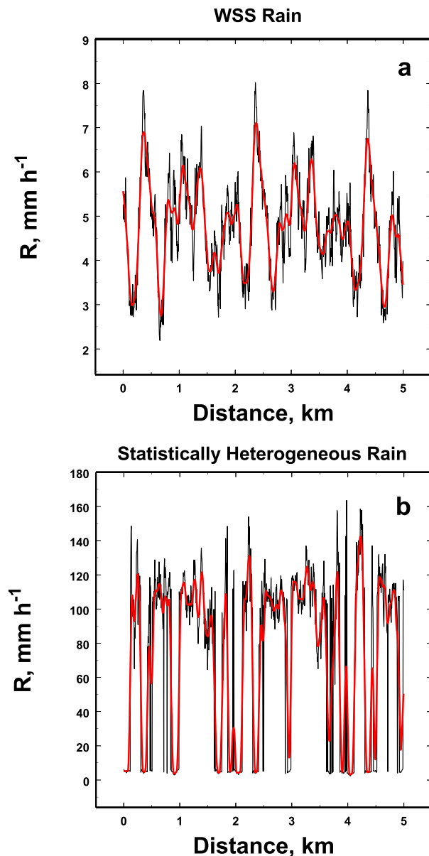
FIG. 11. Two one dimensional examples of synthesized data for (a) WSS data having \alpha = 2 , RD_\alpha = 0.41 , and N_c = 1 so that IXH = 0 and for (b) statistically heterogeneous data having \alpha = 14 , RD_\alpha = 2.90 , and N_c = 2 , so that IXH = 1.70 in agreement with the input assumptions in both cases. As before, the red line denotes the WLSE local regression fit spanning twice the decorrelation length.
