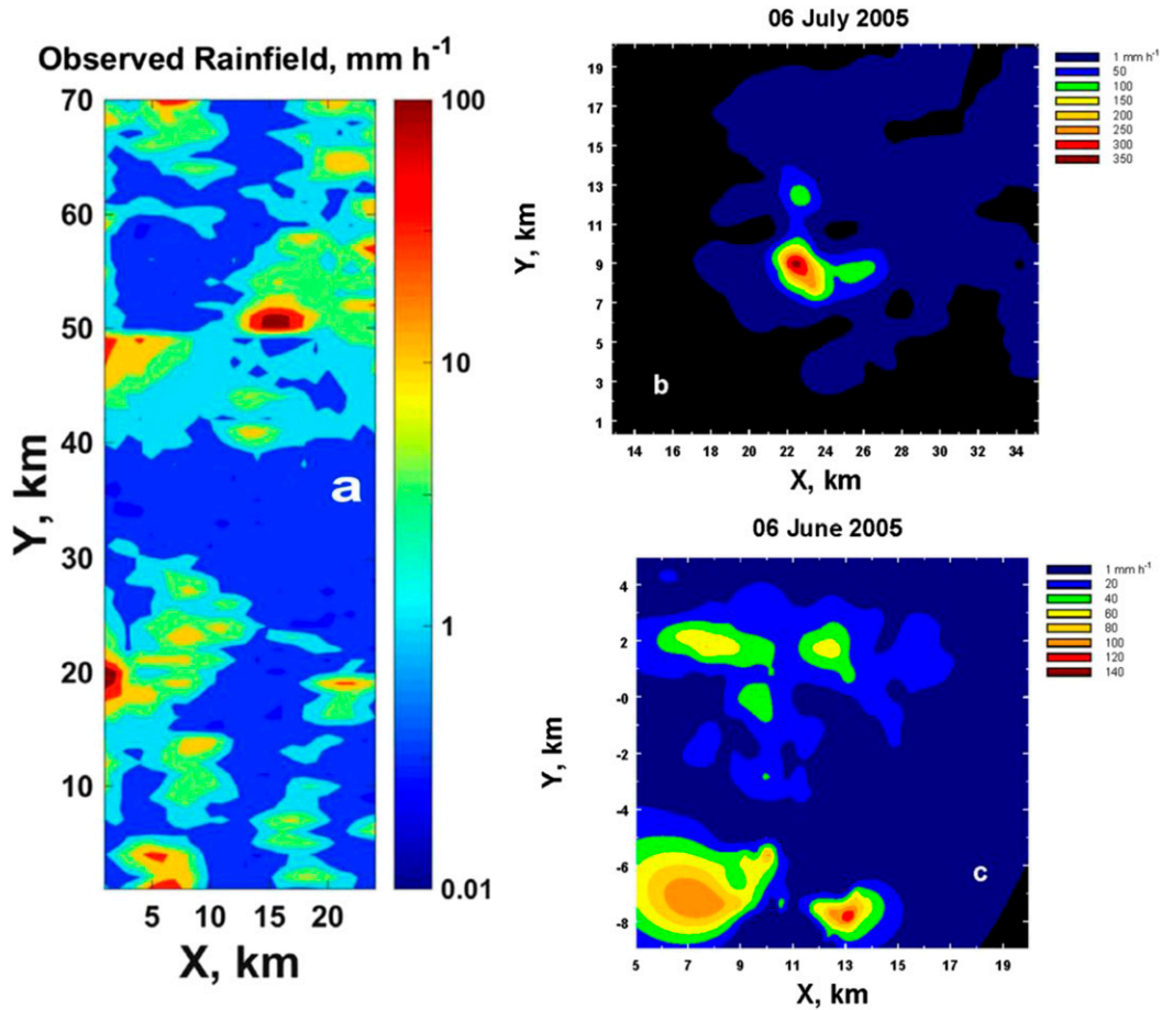
FIG. 13. Examples of rainfall rate estimated from the radar reflectivity. (a) For these data, RD_\alpha = 0 and N_c = 2 . Hence, IXH = 0.5 , so these data are statistically heterogeneous, but they may be considered to be a statistical mixture because RD_\alpha = 0 . (b) In this case RD_\alpha = 2.29 and N_c = 3 . Consequently, IXH = 1.26 , so these data are statistically heterogeneous. (c) As in Fig. 12b, but for a different storm. While RD_\alpha = 0.232 is small, N_c = 4 , so IXH = 1.5 . These data, therefore, exhibit statistical heterogeneity because of different contributing components, but they may also almost be considered to be a statistical mixture.
